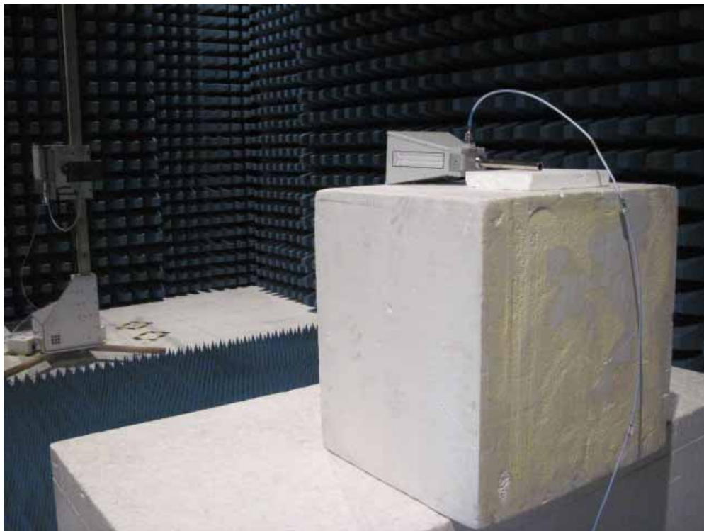
Description: Substitution Antenna for Spurious Emission Above 1G Test
