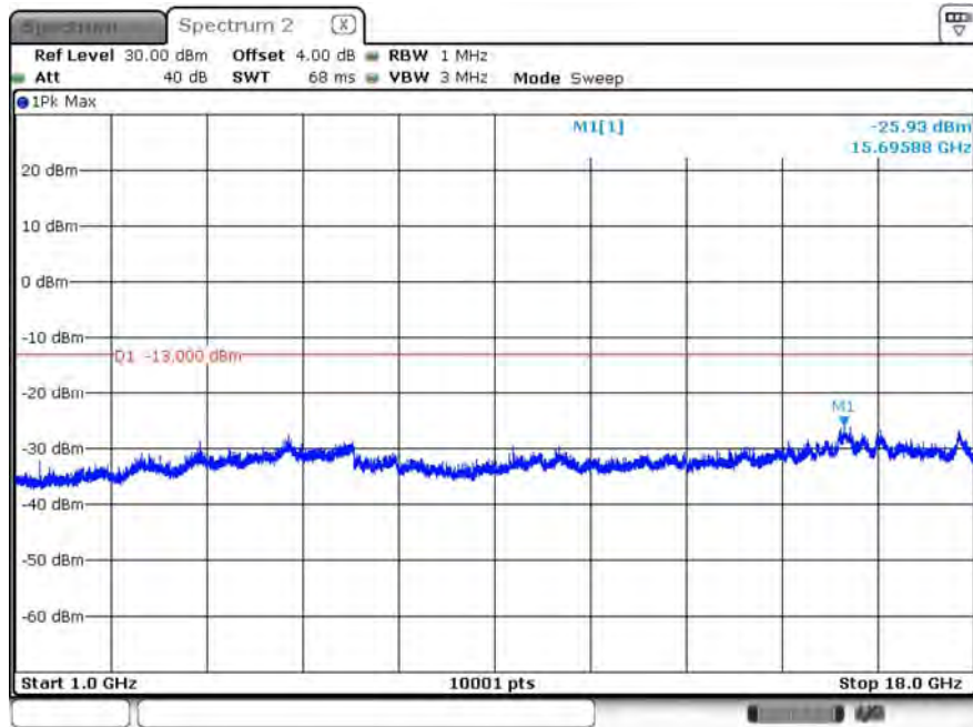
B12_CH23155_5M_1RB12_16-QAM_Above 1G
