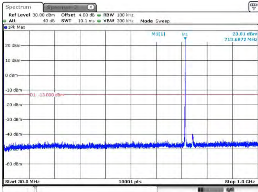
B12_CH23155_5M_1RB12_16-QAM_Below 1G
