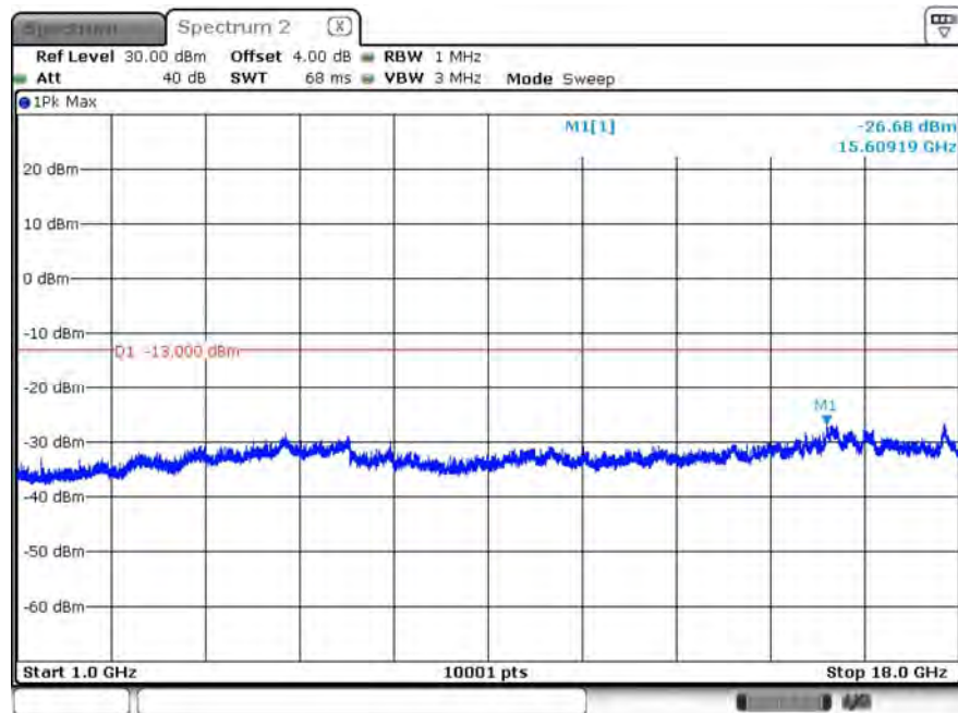
B12_CH23130_10M_1RB24_16-QAM_Above 1G
