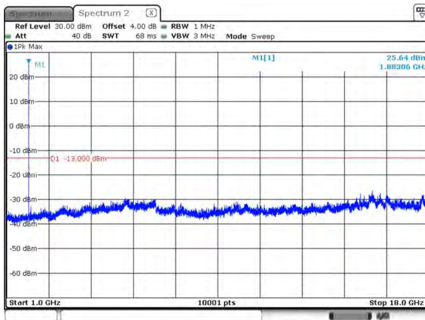
B25_CH26365_10M_1RB24_16-QAM_Above 1G
