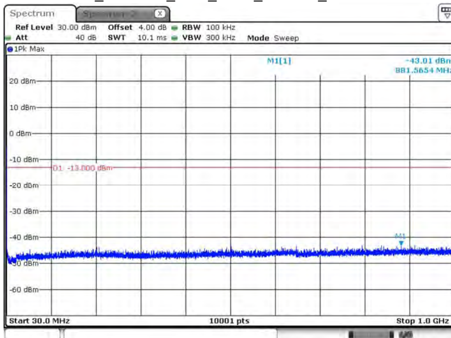
B25_CH26365_1.4M_1RB2_16-QAM_Below 1G
