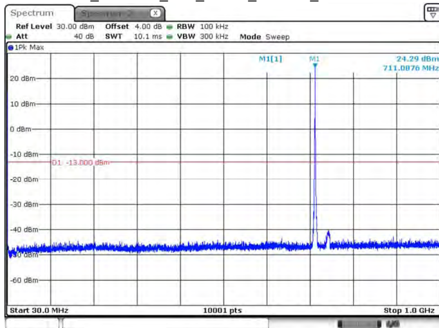
B12_CH23130_10M_1RB24_16-QAM_Below 1G
