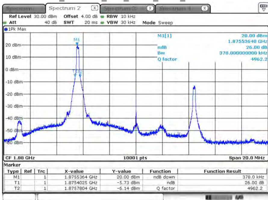
B2_CH18900_10M_QPSK_1RB0_26dB BW
