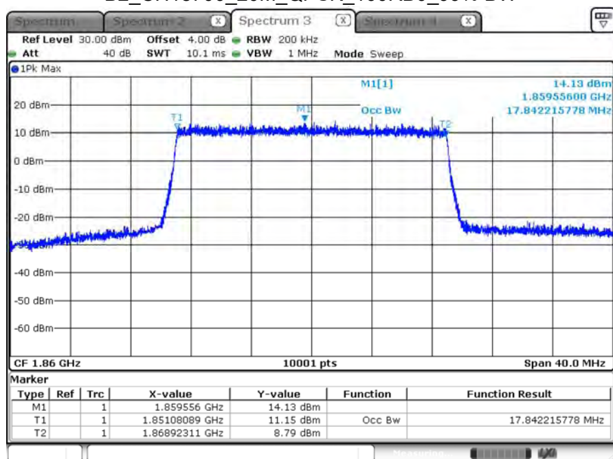
B2_CH18700_20M_QPSK_100RB0_99% BW
