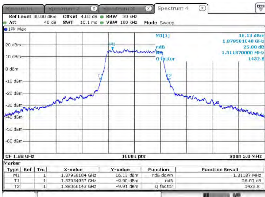
B2_CH18900_1.4M_16-QAM_6RB0_26dB BW
