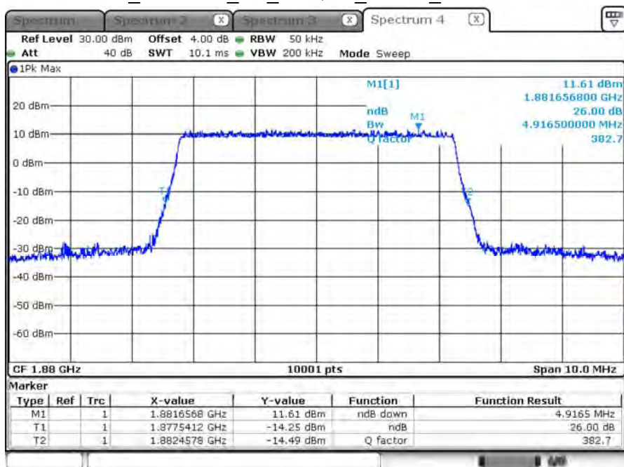
B2_CH18900_5M_16-QAM_25RB0_26dB BW
