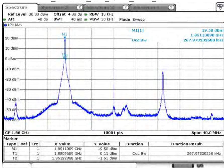
B2_CH18700_20M_QPSK_1RB0_99% BW
