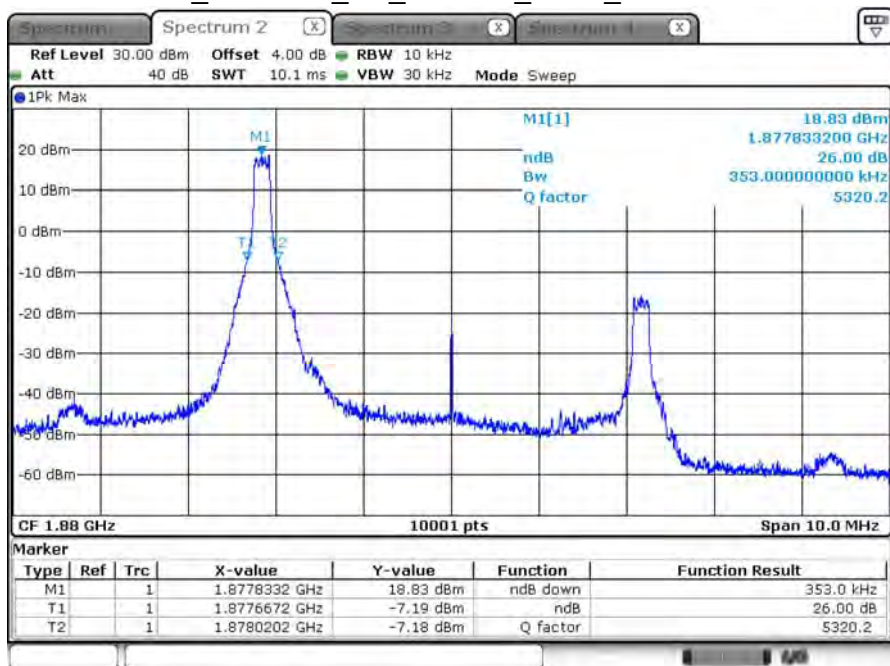
B2_CH18900_5M_16-QAM_1RB0_26dB BW
