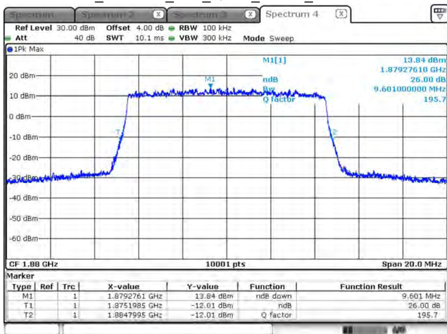
B2_CH18900_10M_QPSK_50RB0_26dB BW
