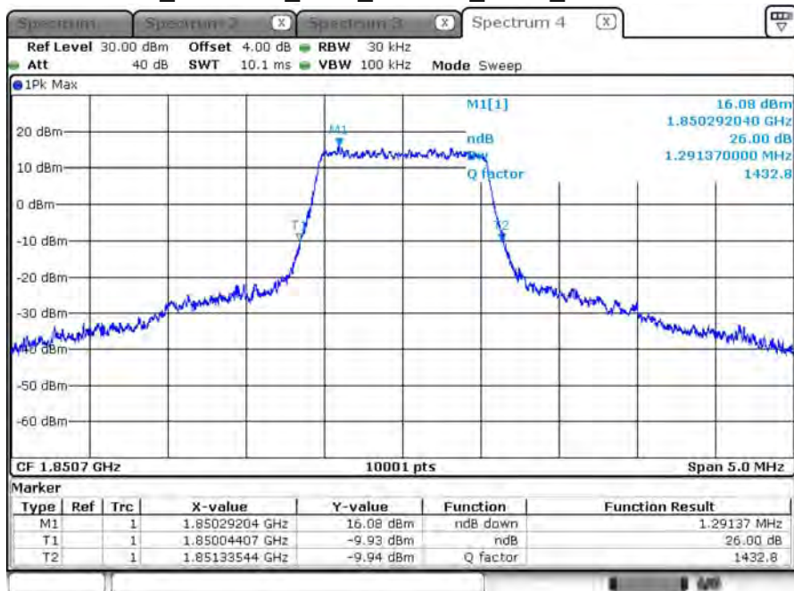
B2_CH18607_1.4M_16-QAM_6RB0_26dB BW
