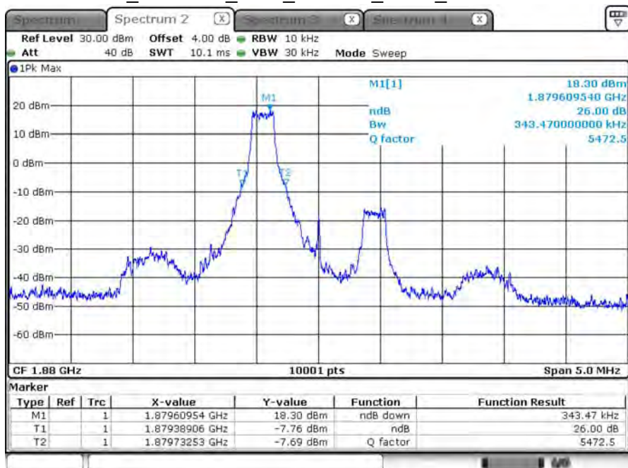
B2_CH18900_1.4M_16-QAM_1RB0_26dB BW
