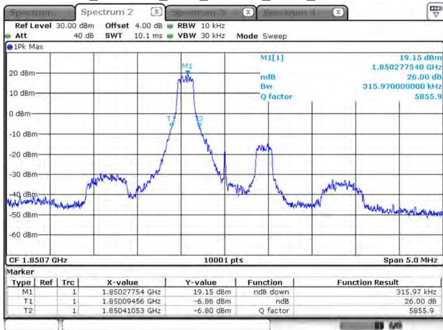
B2_CH18607_1.4M_16-QAM_1RB0_26dB BW
