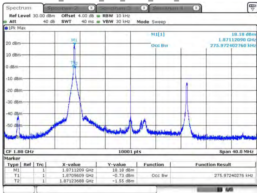
B2_CH18900_20M_QPSK_1RB0_99% BW
