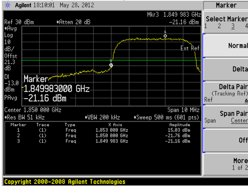
Plot 7.4.11) WCDMA; PCS low channel, below 1850 MHz
