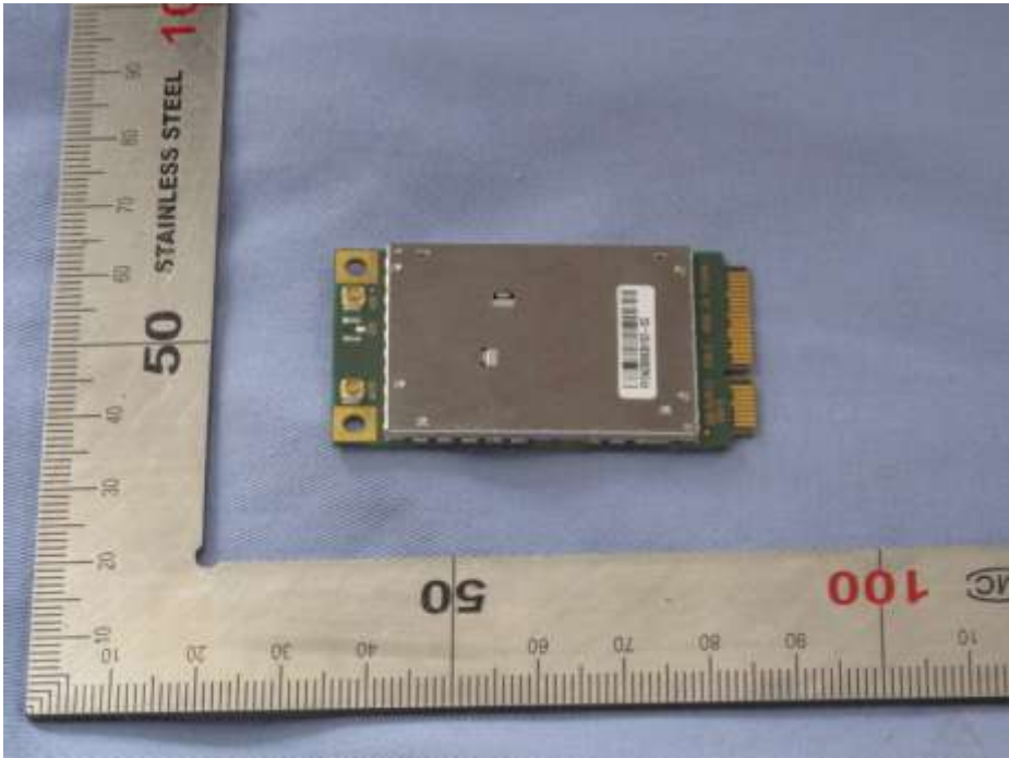
MC8805 Front
