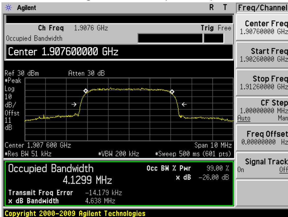
Figure Channel 9538 (1907.6MHz)
