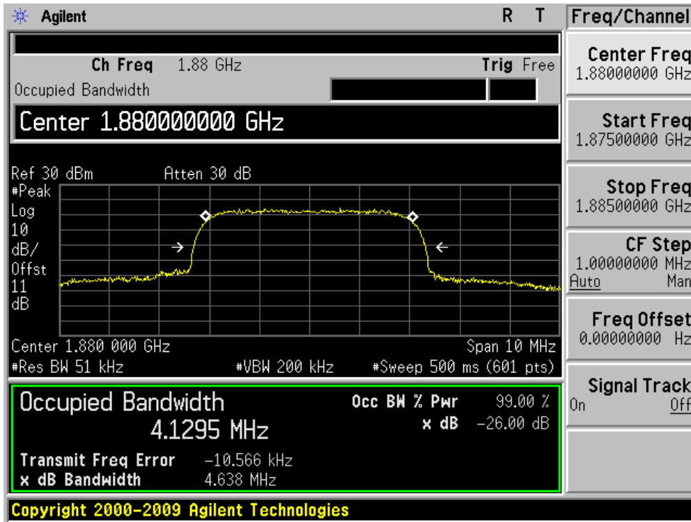
Figure Channel 9400 (1880.0MHz)
