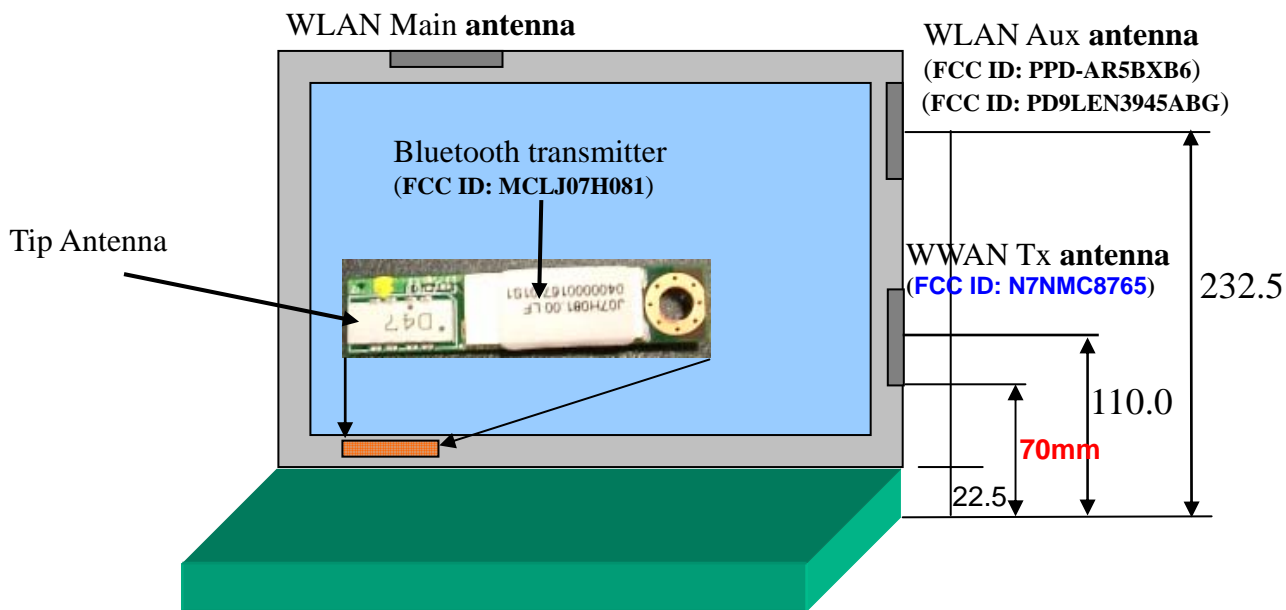
Figure-1 Antenna assembly of T60 series
