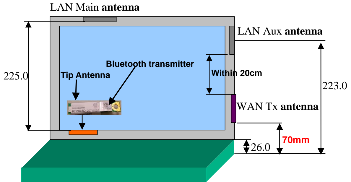
Figure-1 Antenna assembly of Z61m series
