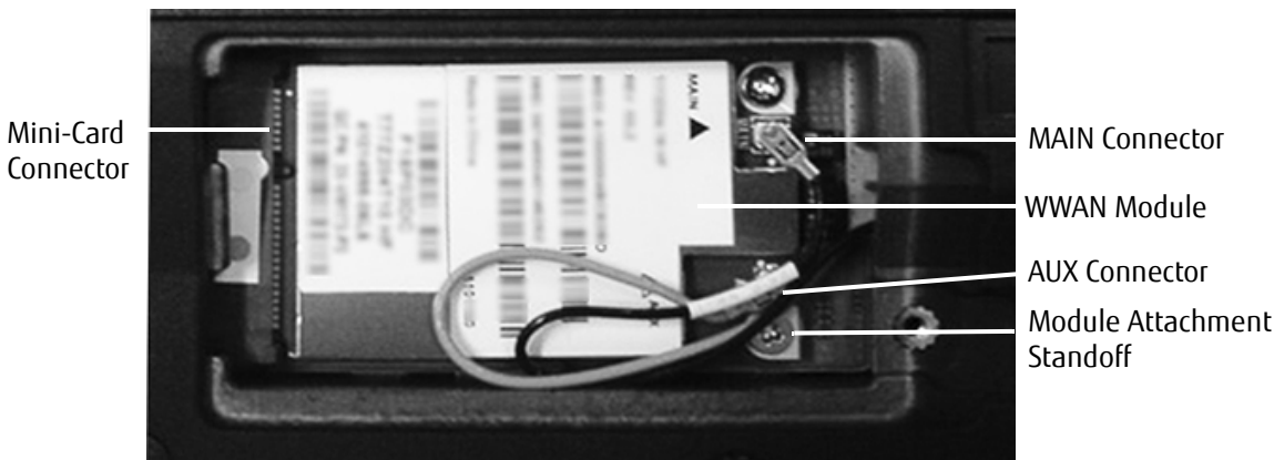
Figure 2. Module attachment standoff
