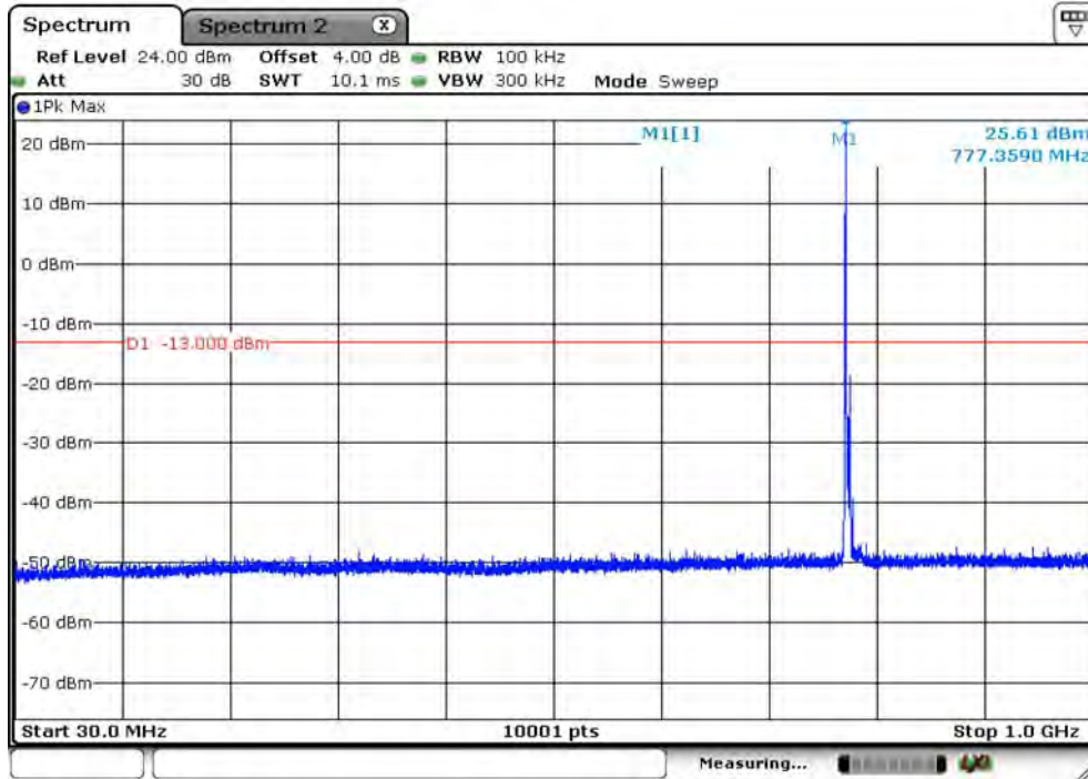
B13_CH23205_5M_1RB0_QPSK_Below 1G
