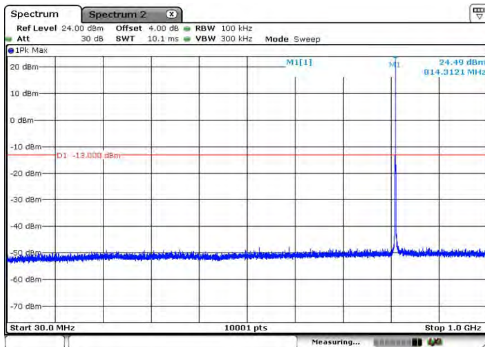
B26_CH26697_1.4M_1RB0_QPSK_Below 1G
