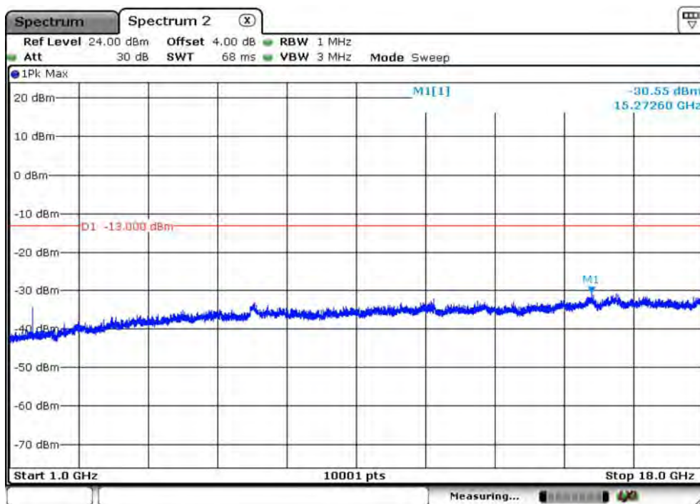
B13_CH23205_5M_1RB0_QPSK_Above 1G
