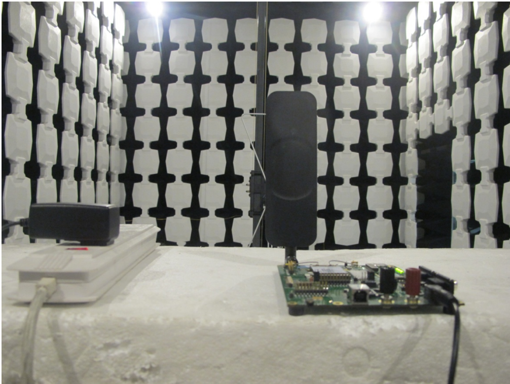
Pic1. Receiver spurious emissions
