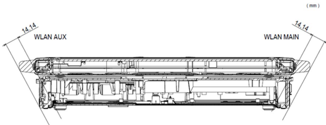
Location of the antennas relative to the protrusions and rear.
