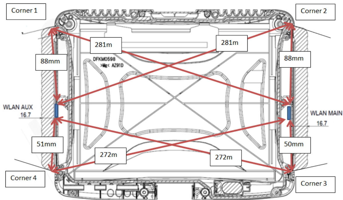
Location of the Antennas relative to the indented corners
