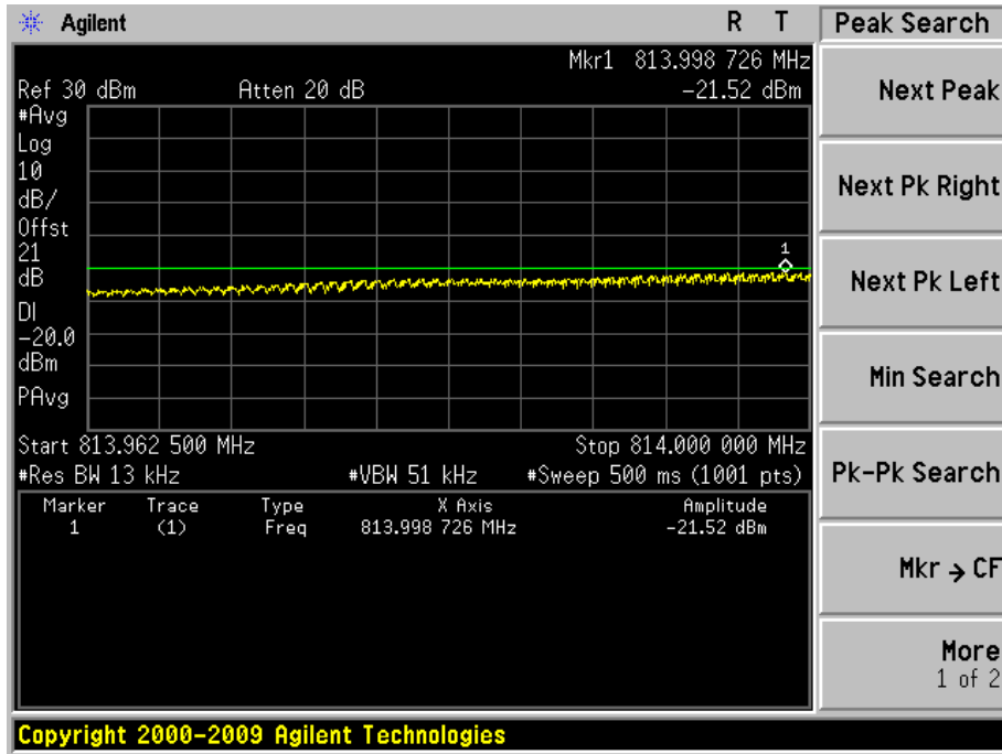
Figure Channel 26697 (814.70MHz) 1RB0
