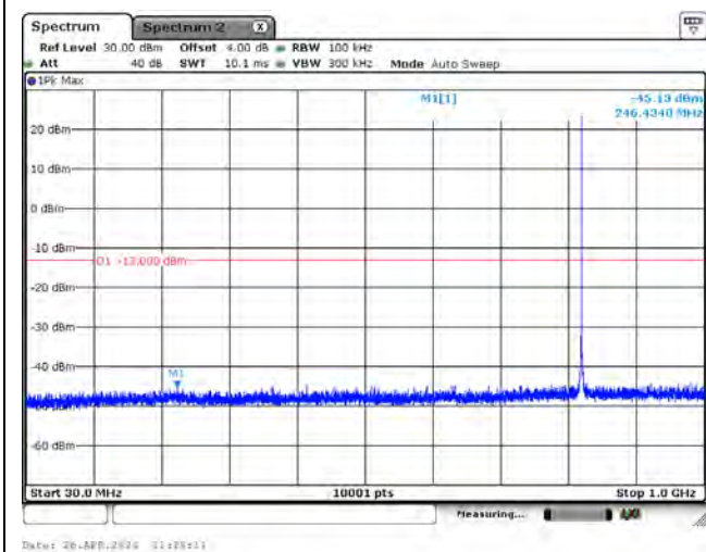
CH26792_3.75k_QPSK_1RB0_Below 1G
