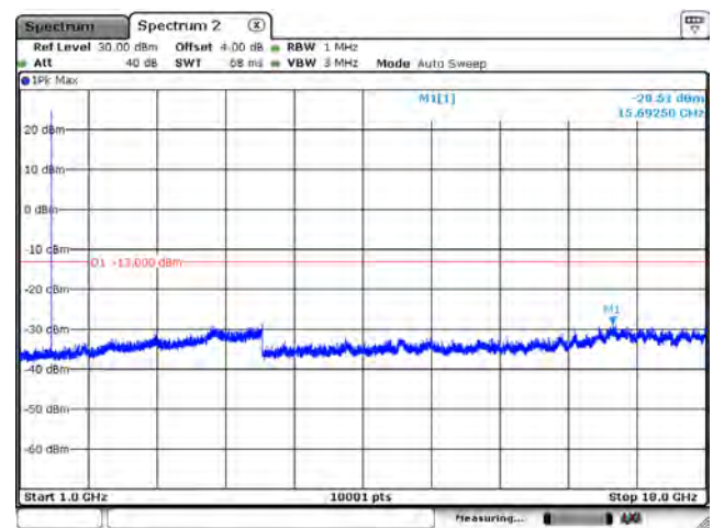
CH132670_15k_QPSK_1RB0_Above 1G
