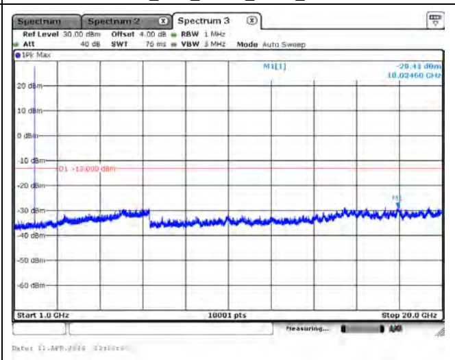
CH26590_20M_QPSK_1RB0_Above 1G
