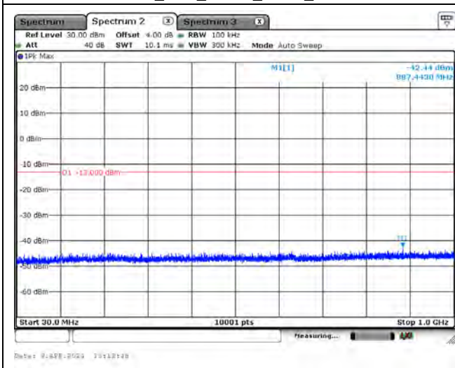
CH26590_20M_QPSK_1RB0_Below 1G
