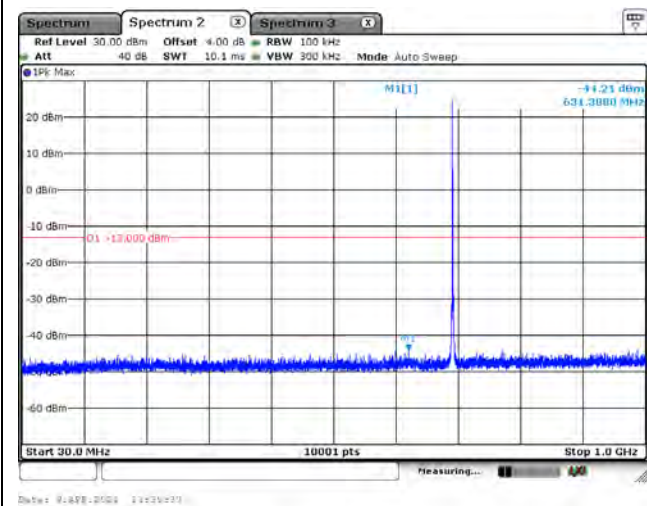
CH23095_5M_QPSK_1RB0_Below 1G
