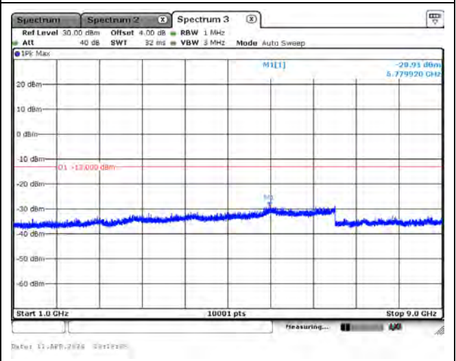
CH27025_3M_QPSK_1RB0_Above 1G
