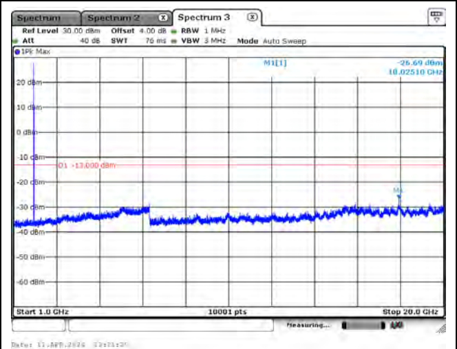
CH26365_10M_QPSK_1RB0_Above 1G
