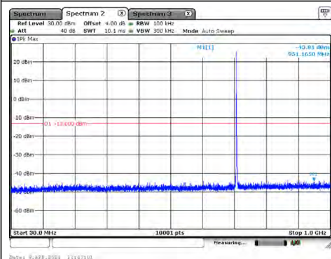
CH23130_10M_QPSK_1RB0_Below 1G
