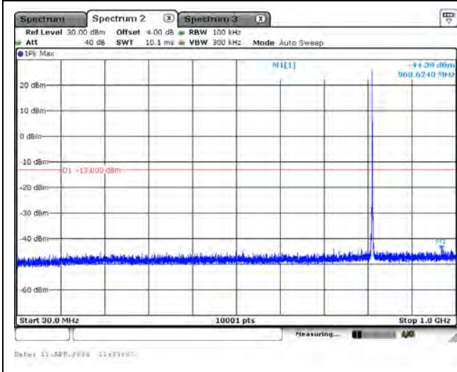
CH26740_10M_QPSK_1RB0_low_Below 1G
