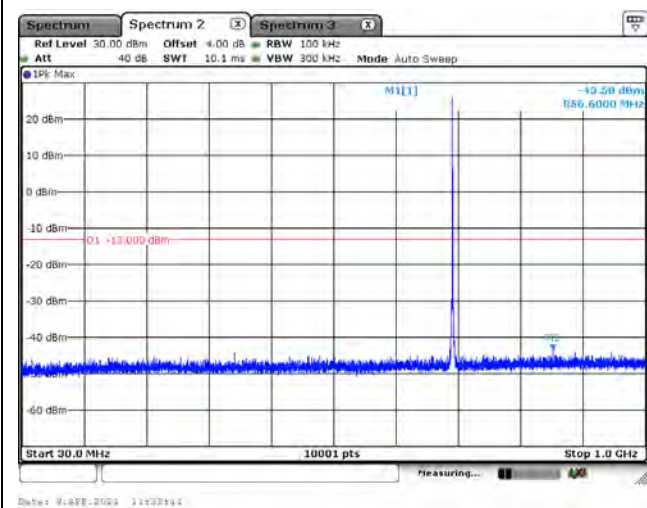
CH23095_3M_QPSK_1RB0_Below 1G
