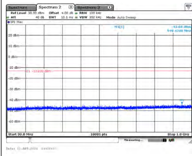
CH132322_15M_QPSK_1RB0_Below 1G
