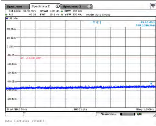
CH26365_20M_QPSK_1RB0_Below 1G
