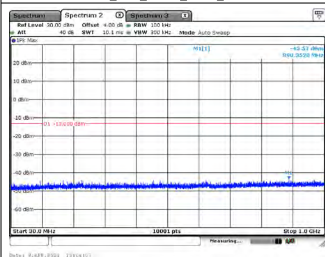
CH26615_15M_QPSK_1RB0_Below 1G
