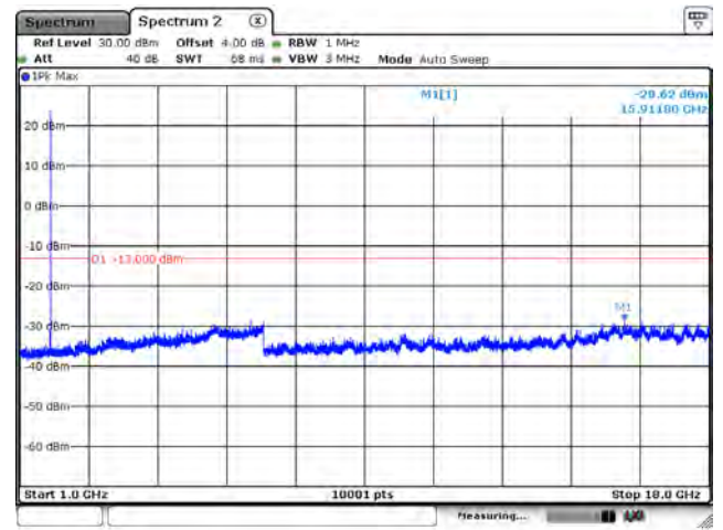
CH132322_15k_BPSK_1RB0_Above 1G
