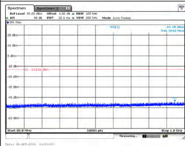
CH133120_3.75k_QPSK_1RB0_Below 1G
