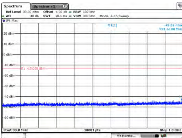
CH26365_15k_QPSK_1RB0_Below 1G
