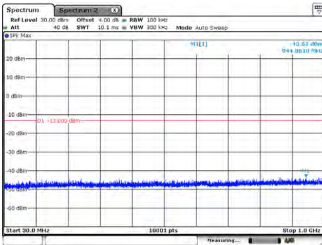
CH26042_15k_QPSK_1RB0_Below 1G
