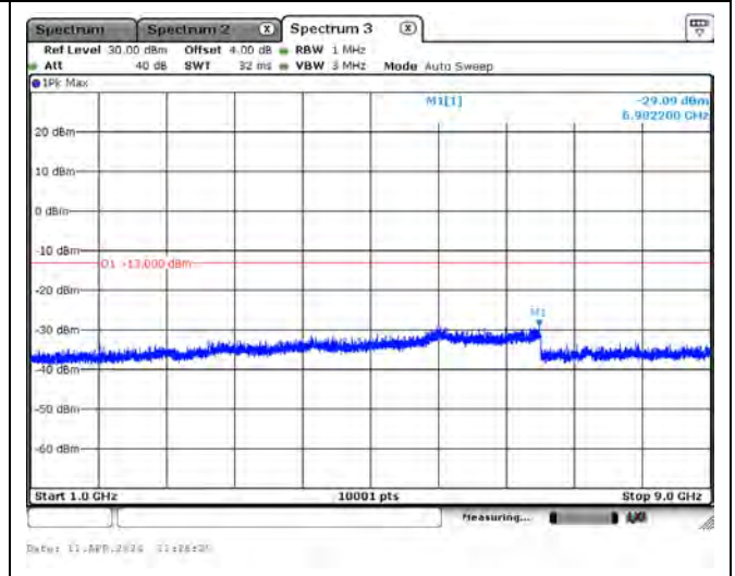
CH26740_10M_QPSK_1RB0_low_Above 1G
