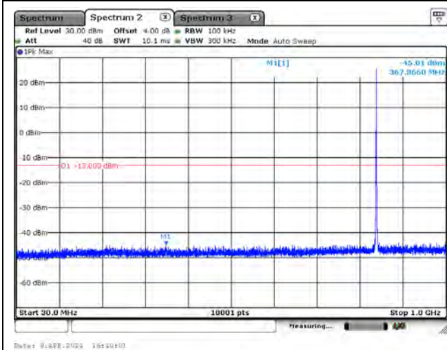
CH26915_15M_QPSK_1RB0_Below 1G
