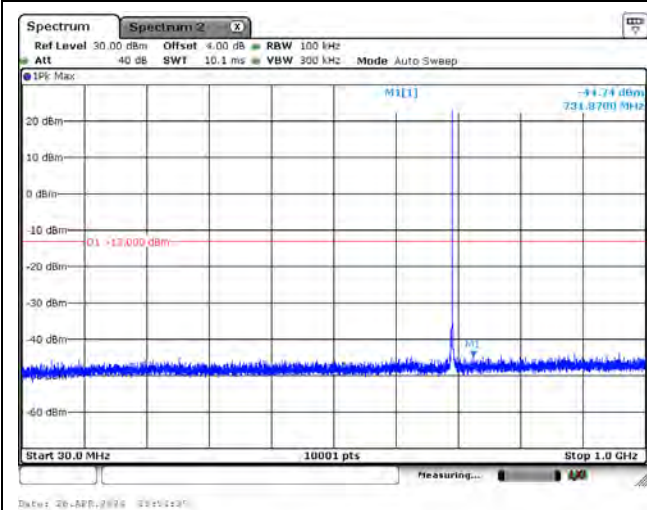
CH23012_15k_BPSK_1RB0_Below 1G
