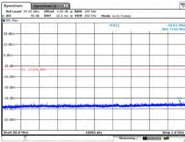
CH132322_15k_BPSK_1RB0_Below 1G
