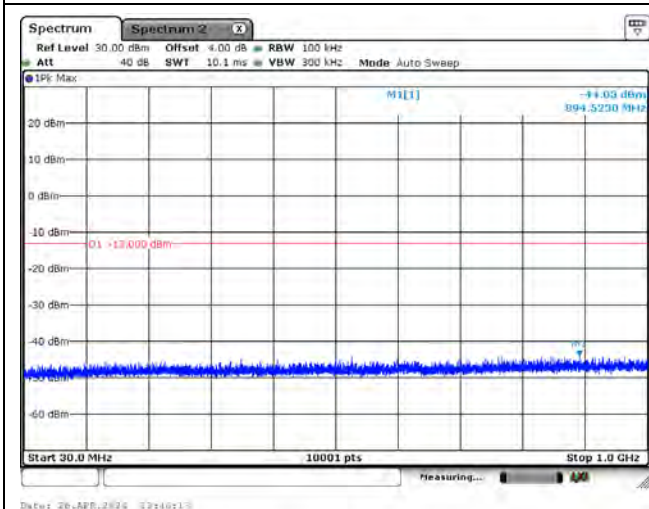
CH132670_3.75k_QPSK_1RB0_Below 1G
