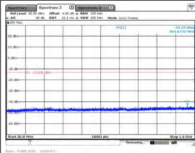
CH26365_10M_QPSK_1RB0_Below 1G
