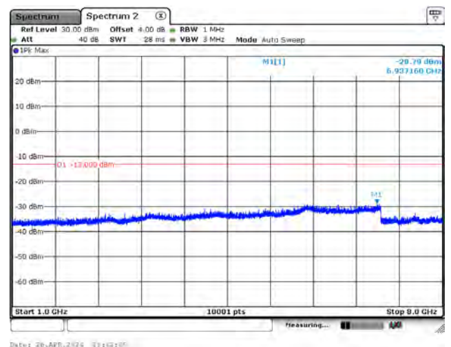
CH23278_15k_BPSK_1RB0_Above 1G
