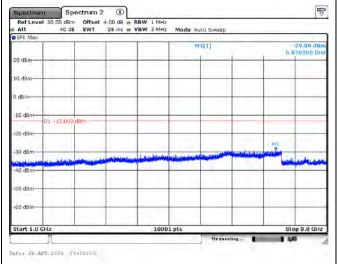
CH134092_15k_BPSK_1RB0_Above 1G
