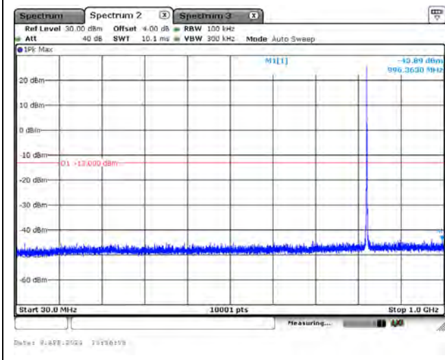
CH26915_3M_QPSK_1RB0_Below 1G
