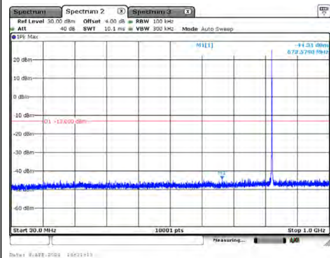
CH26915_10M_QPSK_1RB0_Below 1G
