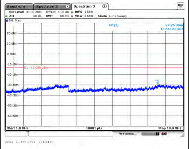
CH132322_3M_QPSK_1RB0_Above 1G
