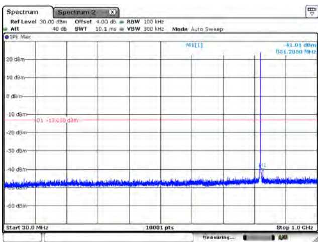
CH26788_15k_BPSK_1RB0_Below 1G
