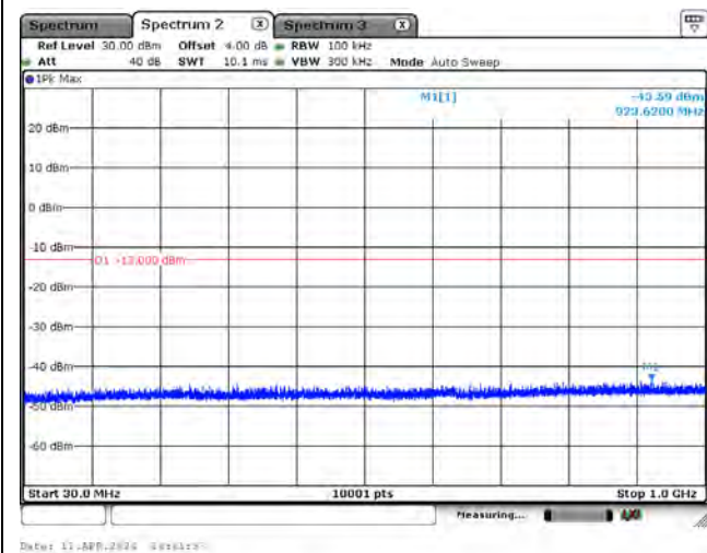
CH132322_20M_QPSK_1RB0_Below 1G
