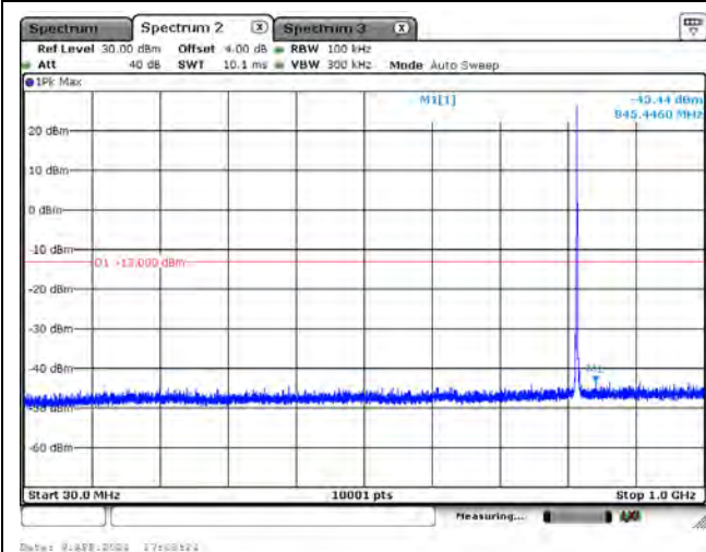
CH26775_3M_QPSK_1RB0_Below 1G
