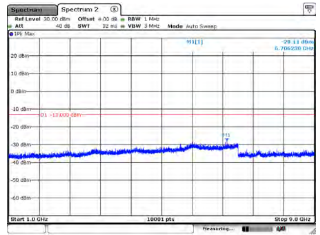
CH26692_15k_BPSK_1RB0_Above 1G
