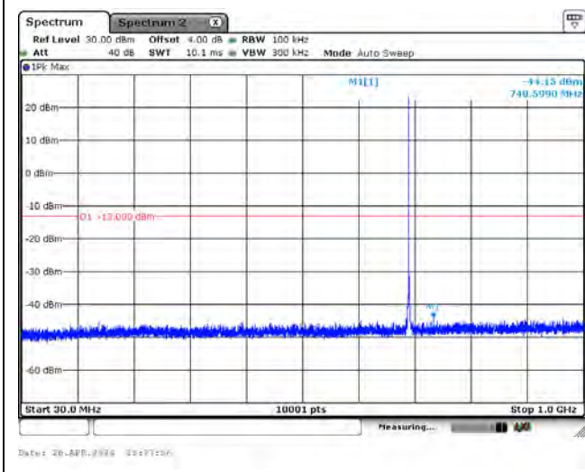
CH134092_15k_BPSK_1RB0_Below 1G
