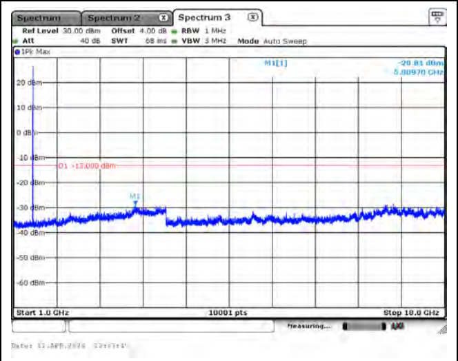
CH132657_3M_QPSK_1RB0_Above 1G
