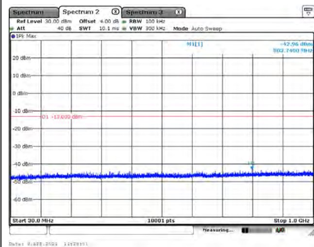
CH26065_5M_QPSK_1RB0_Below 1G
