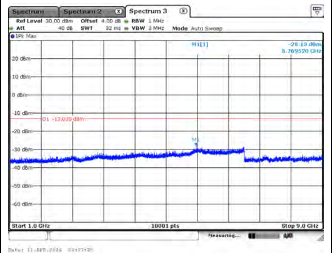
CH26915_10M_QPSK_1RB0_Above 1G
