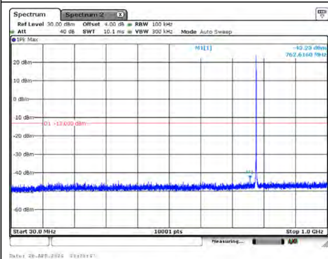
CH23230_15k_QPSK_1RB0_Below 1G
