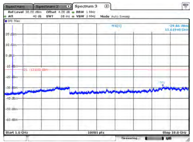
CH132322_10M_QPSK_1RB0_Above 1G
