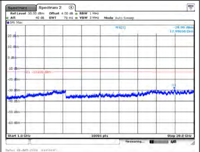
CH26365_15k_BPSK_1RB0_Above 1G
