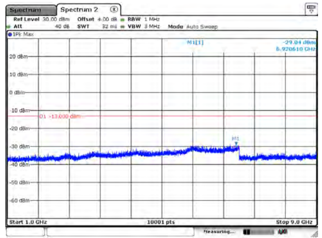
CH26792_15k_BPSK_1RB0_Above 1G
