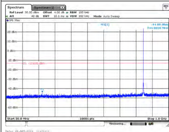
CH27038_3.75k_QPSK_1RB0_Below 1G
