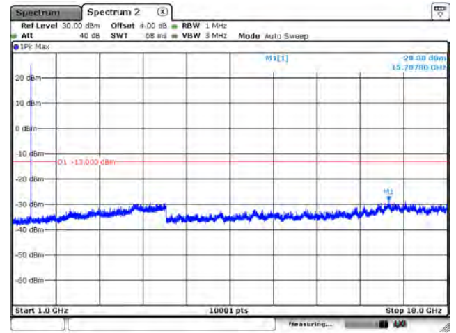
CH131974_15k_BPSK_1RB0_Above 1G
