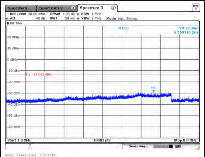
CH23095_3M_QPSK_1RB0_Above 1G
