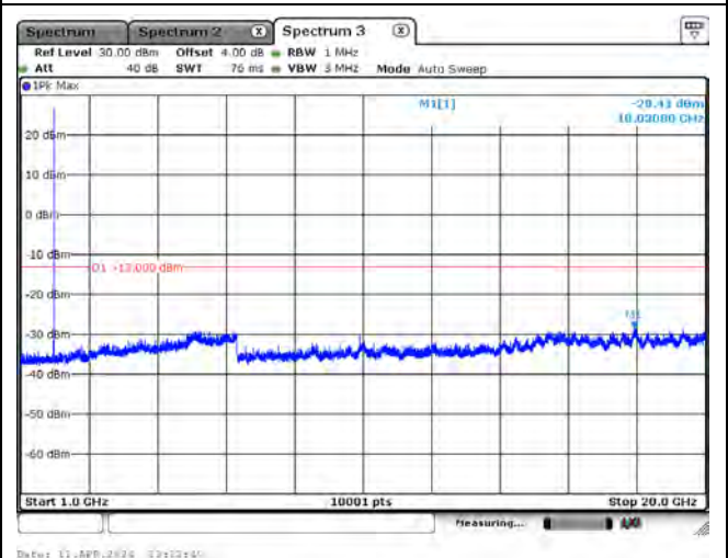
CH26640_10M_QPSK_1RB0_Above 1G
