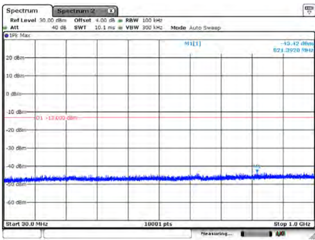
CH132322_15k_QPSK_1RB0_Below 1G
