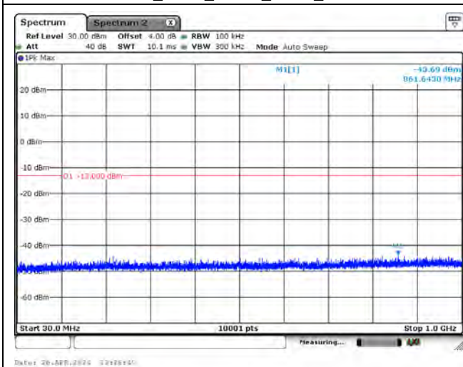
CH26365_3.75k_QPSK_1RB0_Below 1G
