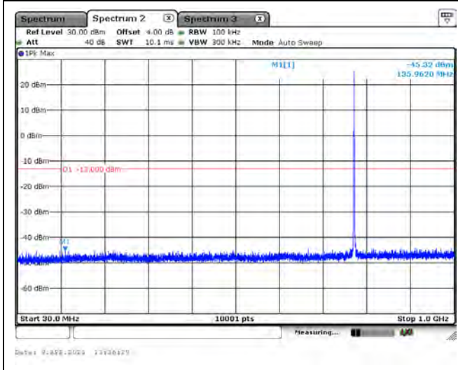
CH23230_5M_QPSK_1RB0_Below 1G
