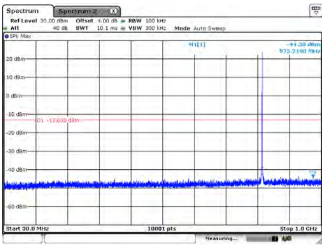
CH26740_15k_BPSK_1RB0_Below 1G
