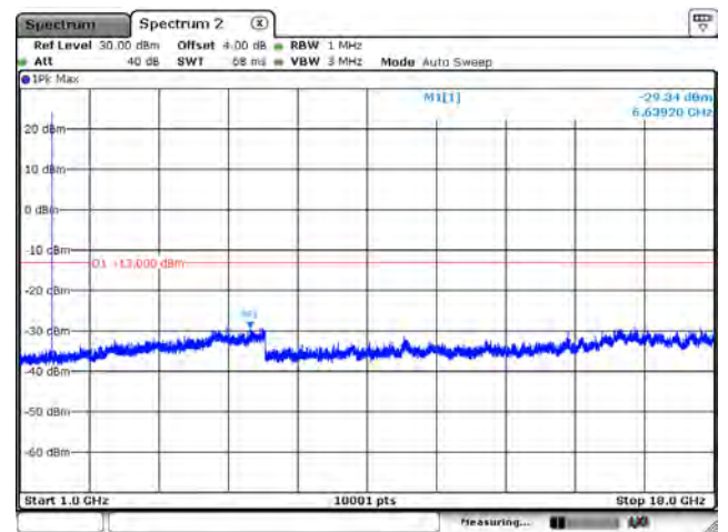
CH132670_15k_BPSK_1RB0_Above 1G
