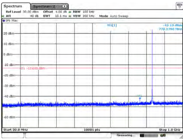
CH26915_15k_QPSK_1RB0_Below 1G
