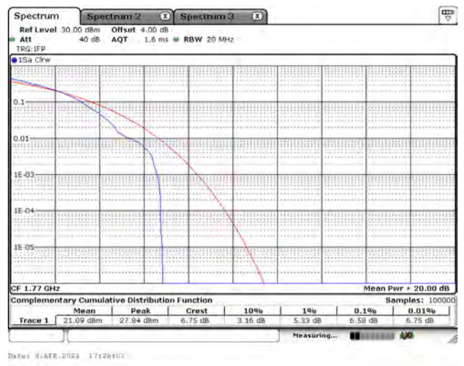
CH132572_20M_16-QAM_1RB5
