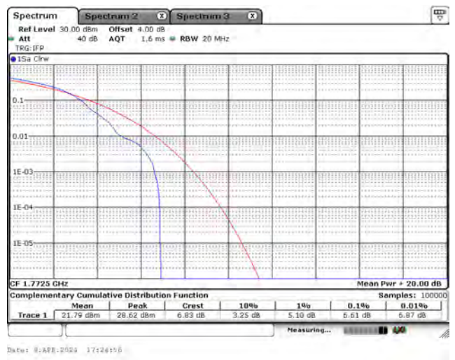
CH132597_15M_16-QAM_1RB5
