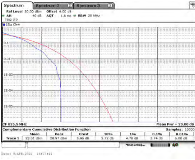
CH27015_5M_QPSK_1RB5
