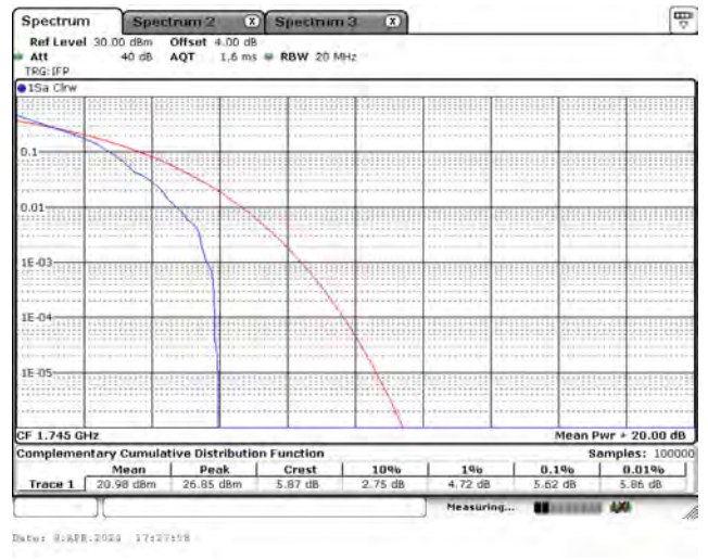
CH132072_20M_16-QAM_1RB0
