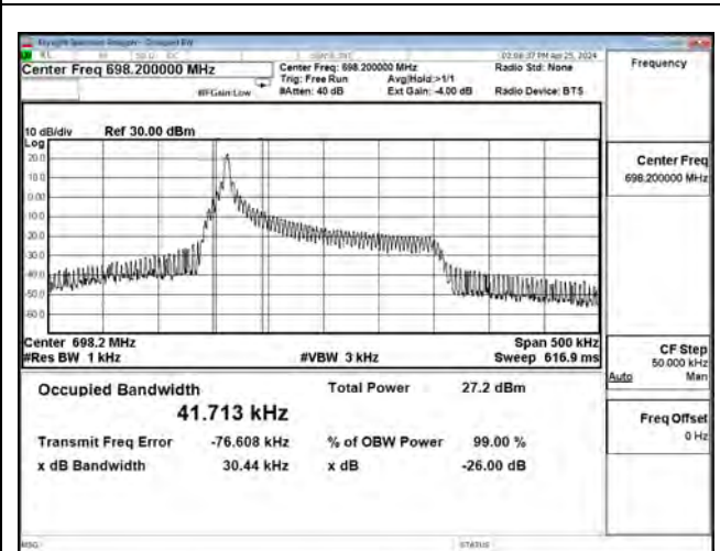
QPSK_CH134004_3.75k_1RB0
