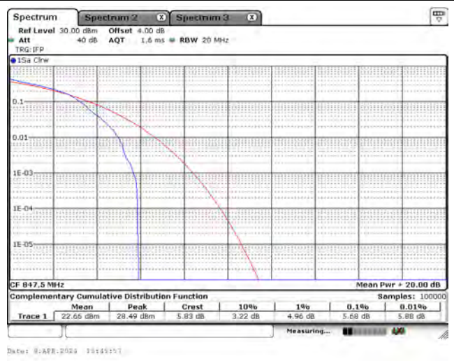
CH27025_3M_16-QAM_1RB5
