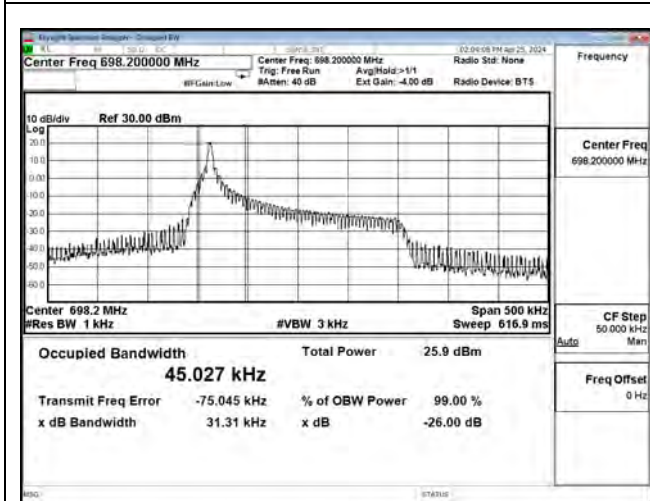
BPSK_CH134004_3.75k_1RB0
