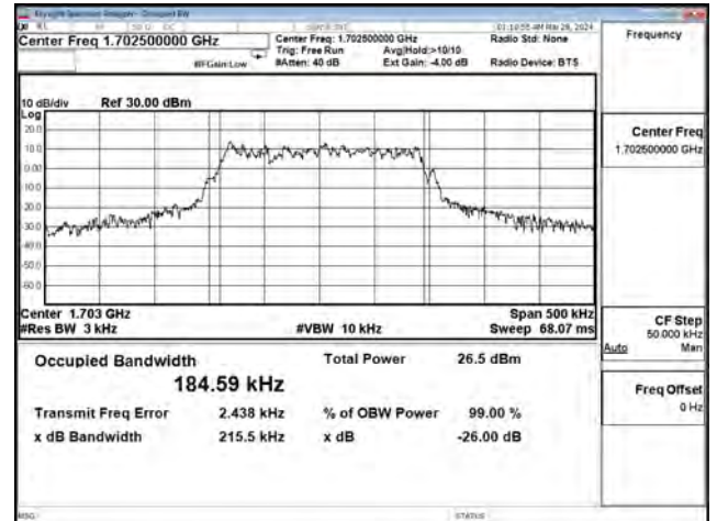
QPSK_CH133047_15k_12RB0
