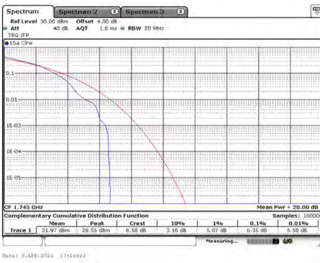
CH132322_15M_16-QAM_1RB0
