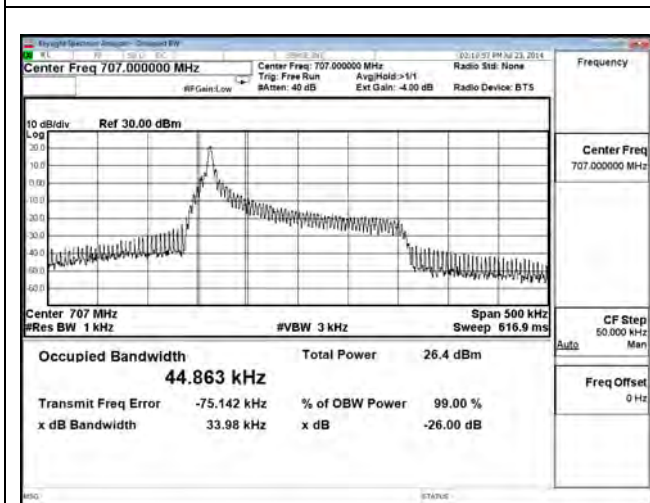
QPSK_CH134092_3.75k_1RB0
