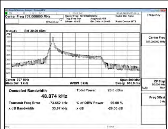
BPSK_CH134092_3.75k_1RB0
