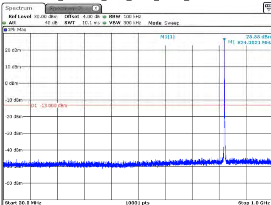
B5_CH20407_1.4M_1RB0_QPSK_Below 1G
