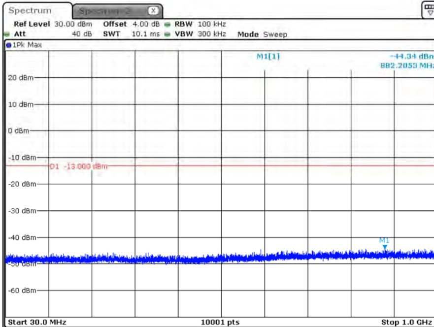
B4_CH19957_1.4M_1RB0_QPSK_Below 1G
