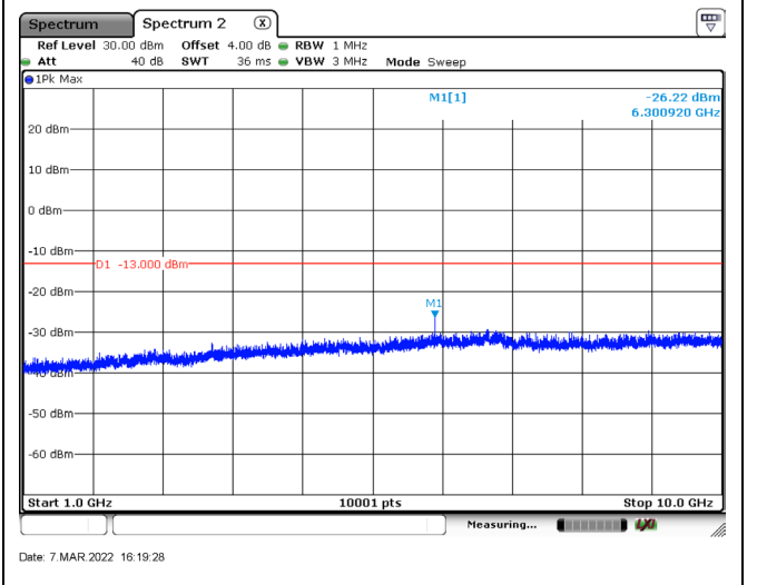
3 MHz / QPSK - Hight / CH21640 / 1RB5 / Above 1 GHz
