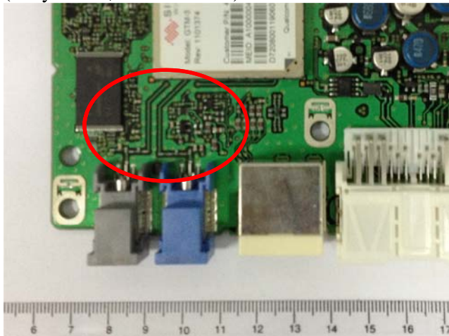
PCB, Antenna circuit details - Deviation from Module Certification (Gray= GPS, Blue=CDMA)
