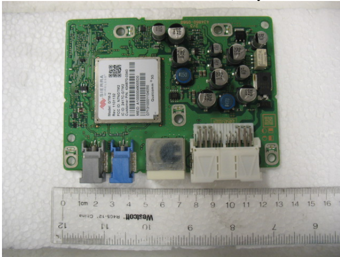
PCB, with module & RF Connections (Gray= GPS, Blue=CDMA)
