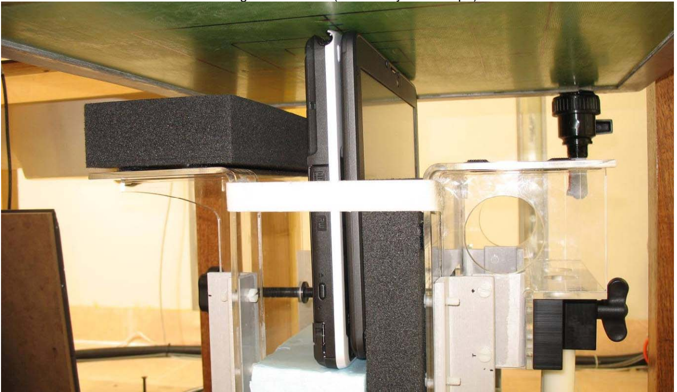
Photo No. 12: Edge On Position (Secondary Landscape) Antenna IN
