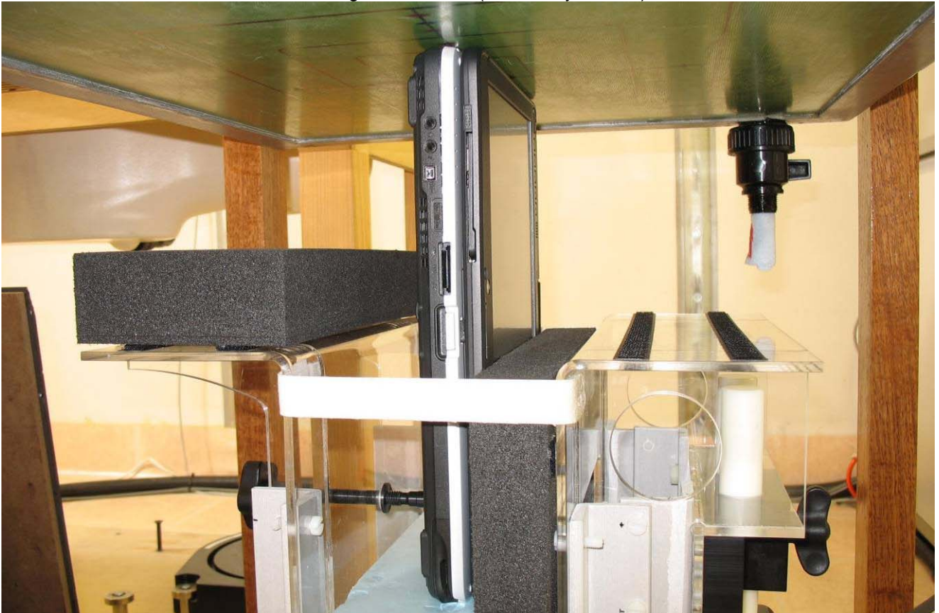
Photo No. 8: Edge On Position (Secondary Portrait) Antenna IN
