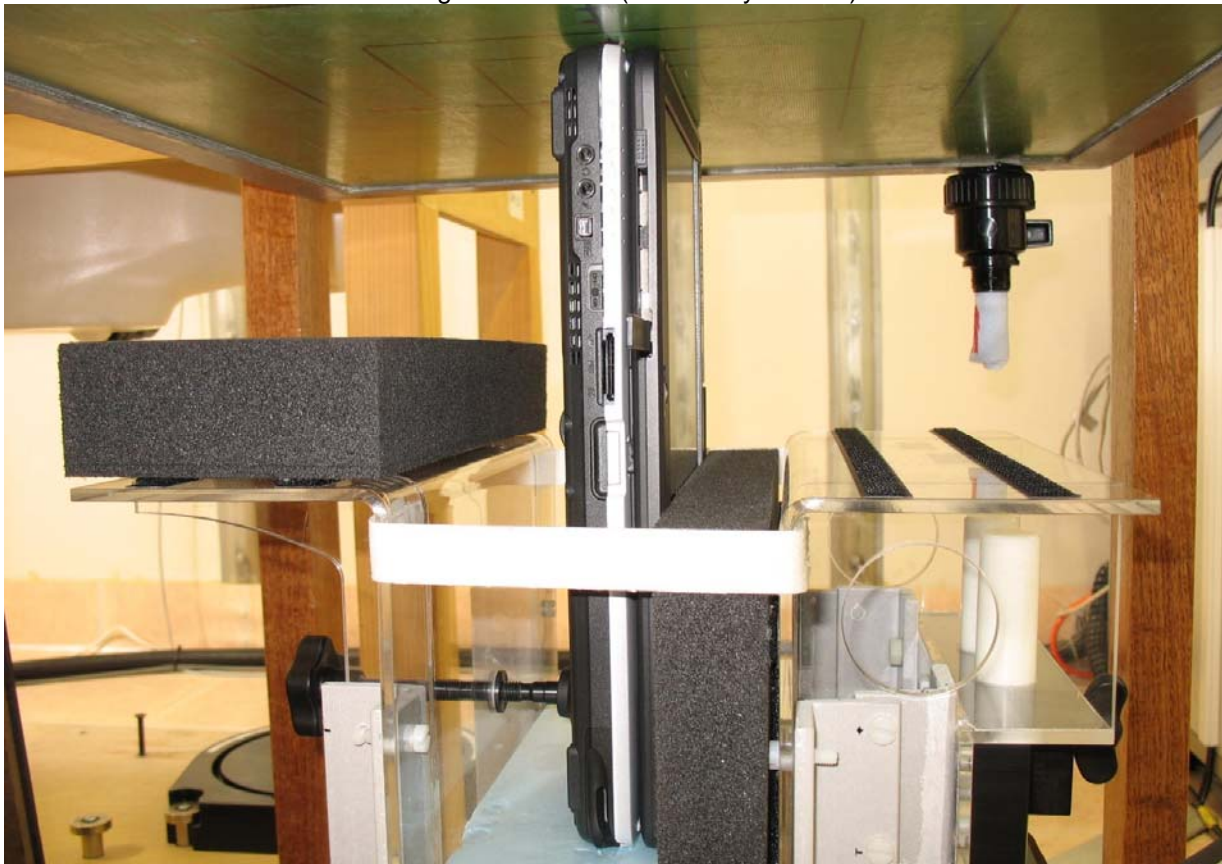
Photo No. 10: Edge On Position (Secondary Portrait) Antenna Out
