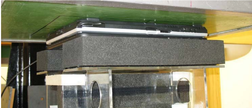
Photo No. 2: Tablet Position Antenna IN
