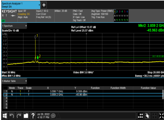
B13_N48(20M)_DFT-s-OFDM_QPSK_Outer_Full_Low_CH
