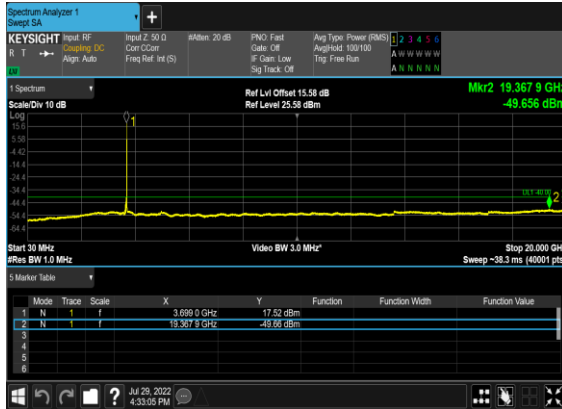
B13_N48(20M)_DFT-s-OFDM_QPSK_Edge_1RB_Right_High_C H
