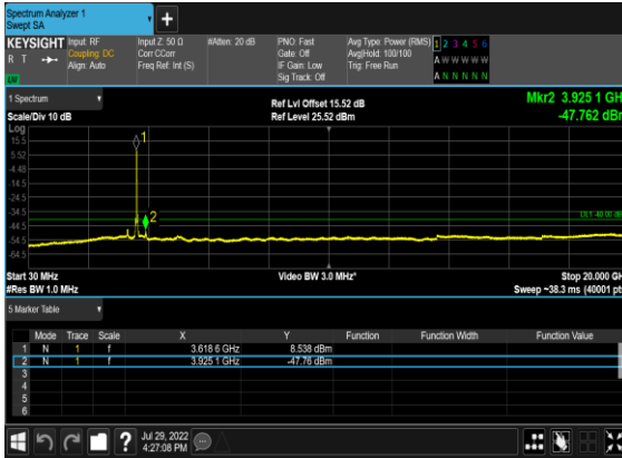
B13_N48(20M)_DFT-s-OFDM_QPSK_Outer_Full_Mid_CH
