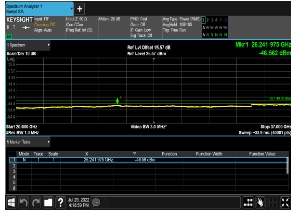
B13_N48(20M)_DFT-s-OFDM_QPSK_Outer_Full_Low_CH
