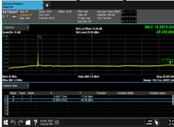
B13_N48(10M)_DFT-s-OFDM_BPSK_Outer_Full_Low_CH
