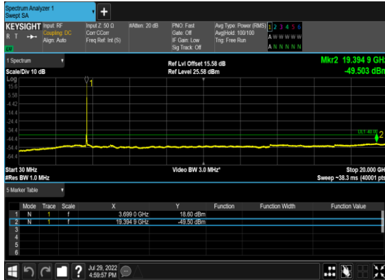
B13_N48(40M)_DFT-s-OFDM_QPSK_Edge_1RB_Right_High_C H
