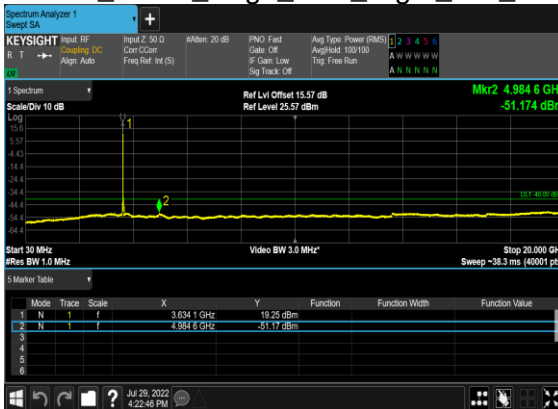
B13_N48(20M)_DFT-s-OFDM_BPSK_Edge_1RB_Right_Mid_CH
