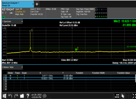
B13_N48(40M)_DFT-s-OFDM_QPSK_Outer_Full_Mid_CH
