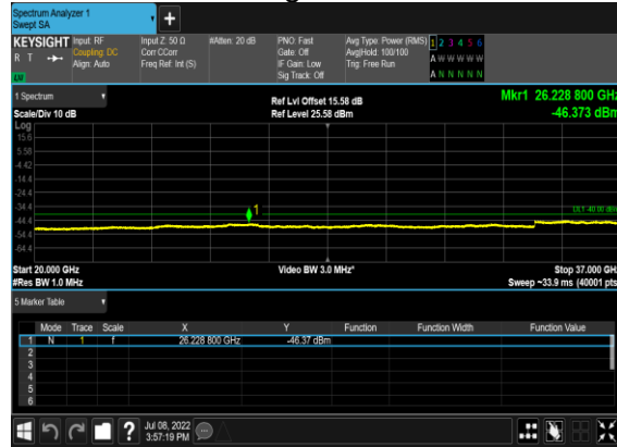
B13_N48(10M)_DFT-s-OFDM_QPSK_Edge_1RB_Left_Mid_CH
