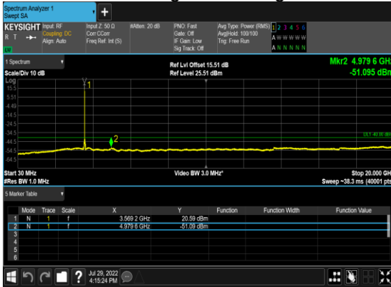
B13_N48(20M)_DFT-s-OFDM_BPSK_Outer_Full_Low_CH
