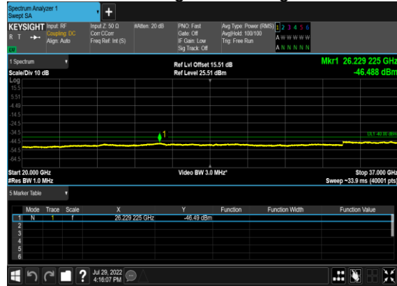
B13_N48(20M)_DFT-s-OFDM_BPSK_Outer_Full_Low_CH
