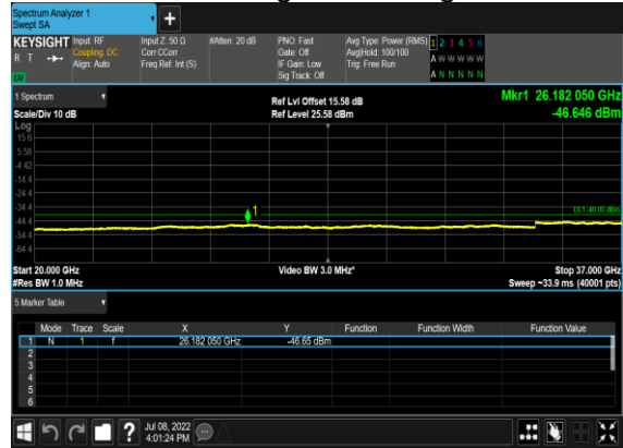
B13_N48(10M)_DFT-s-OFDM_BPSK_Outer_Full_Mid_CH
