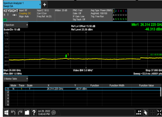
B13_N48(40M)_DFT-s-OFDM_BPSK_Edge_1RB_Right_High_CH
