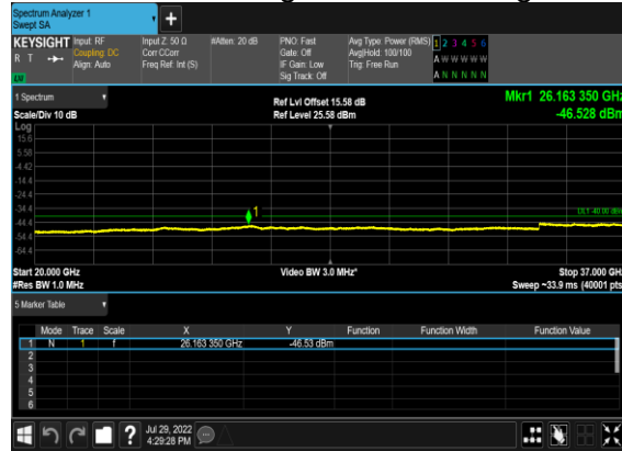
B13_N48(20M)_DFT-s-OFDM_QPSK_Edge_1RB_Left_High_CH
