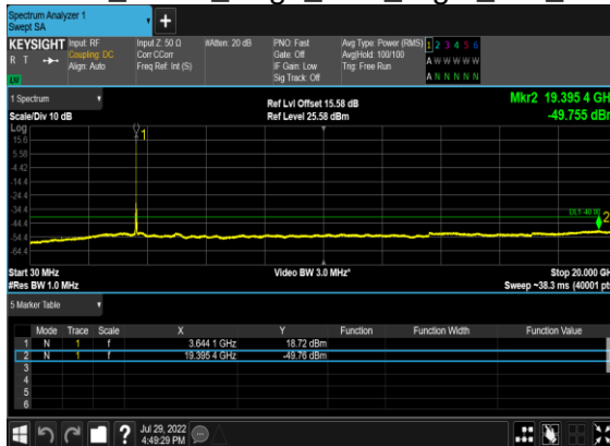
B13_N48(40M)_DFT-s-OFDM_BPSK_Edge_1RB_Right_Mid_CH
