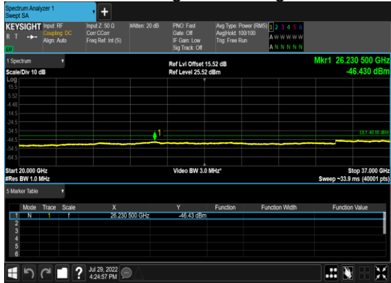
B13_N48(20M)_DFT-s-OFDM_BPSK_Outer_Full_Mid_CH
