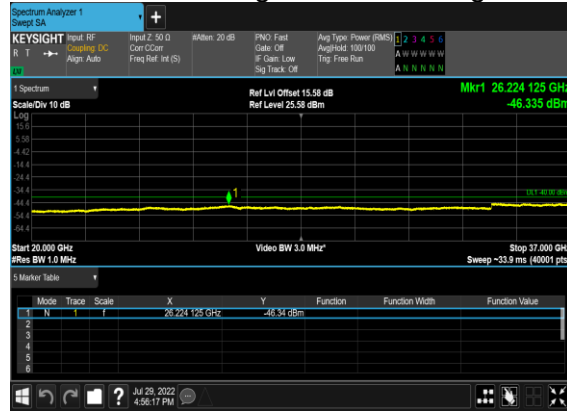
B13_N48(40M)_DFT-s-OFDM_QPSK_Edge_1RB_Left_High_CH
