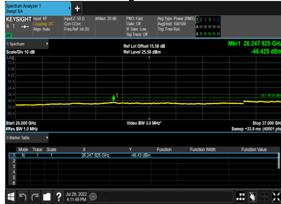
B13_N48(20M)_DFT-s-OFDM_QPSK_Edge_1RB_Left_Low_CH
