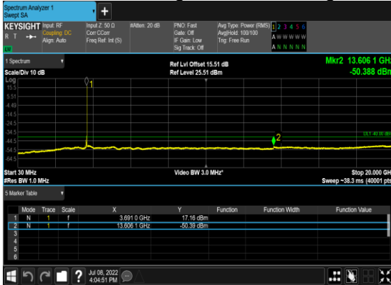
B13_N48(10M)_DFT-s-OFDM_BPSK_Edge_1RB_Right_High_CH
