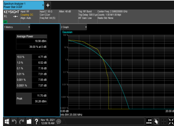
B4_N41(20M)_DFT-s-OFDM_PI_2-BPSK_Edge_1RB_Left_Low_CH
