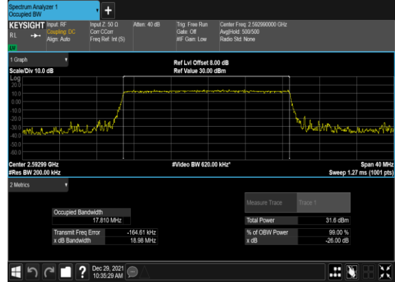
B4_N41(20M)_DFT-s-OFDM_QPSK_Outer_Full_Mid_CH
