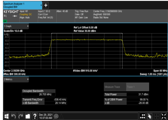
B4_N41(30M)_DFT-s-OFDM_QPSK_Outer_Full_Mid_CH
