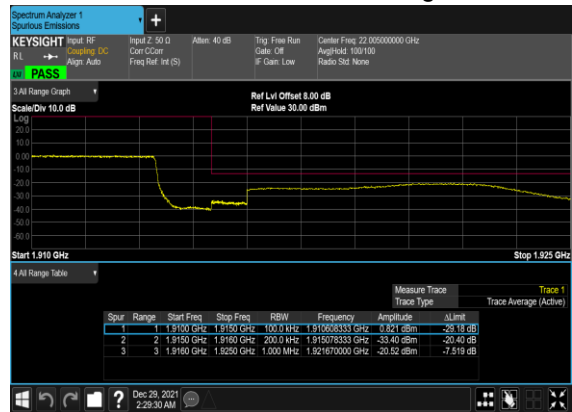
B12_N25(20M)_DFT-s-OFDM_BPSK_Outer_Full_High_CH
