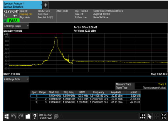
B12_N25(20M)_DFT-s-OFDM_BPSK_Edge_1RB_Right_High_CH
