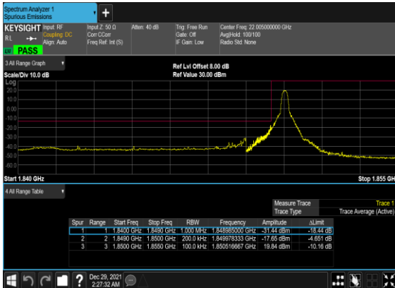
B12_N25(20M)_DFT-s-OFDM_QPSK_Edge_1RB_Left_Low_CH
