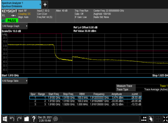
B12_N25(10M)_DFT-s-OFDM_QPSK_Outer_Full_High_CH
