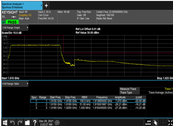
B12_N25(5M)_DFT-s-OFDM_BPSK_Outer_Full_High_CH
