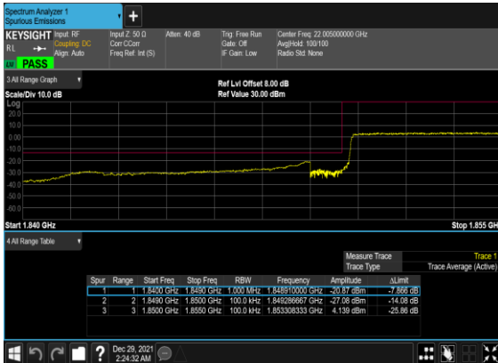
B12_N25(10M)_DFT-s-OFDM_BPSK_Outer_Full_Low_CH
