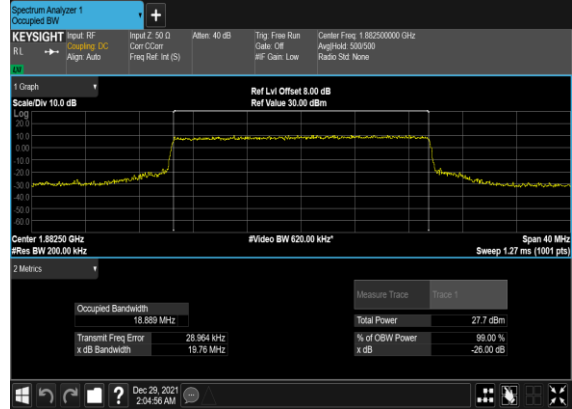
B12_N25(20M)_CP-OFDM_16QAM_Outer_Full_Mid_CH
