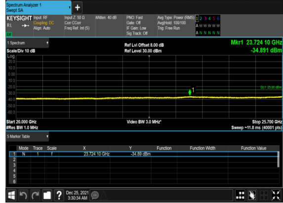
B5_N7(5M)_DFT-s-OFDM_BPSK_Edge_1RB_Left_High_CH
