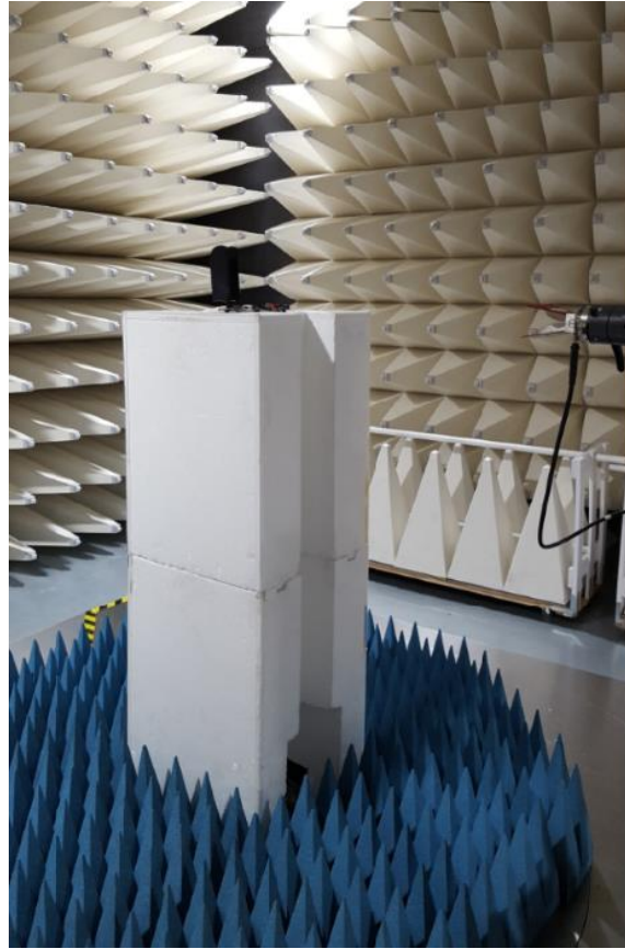
Figure B5. Radiated Setup 3
