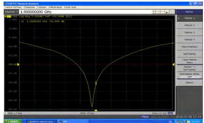
Return Loss-Body
