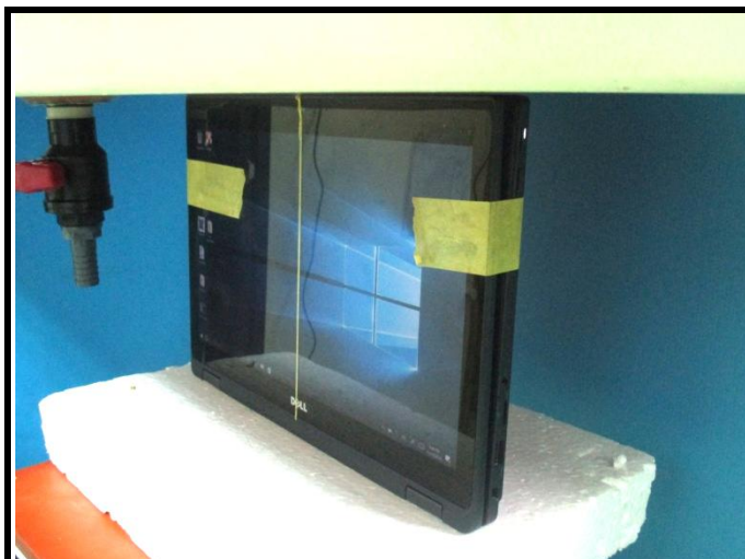
Top Side of EUT with 0 cm Gap (Tablet_Body Mode)
