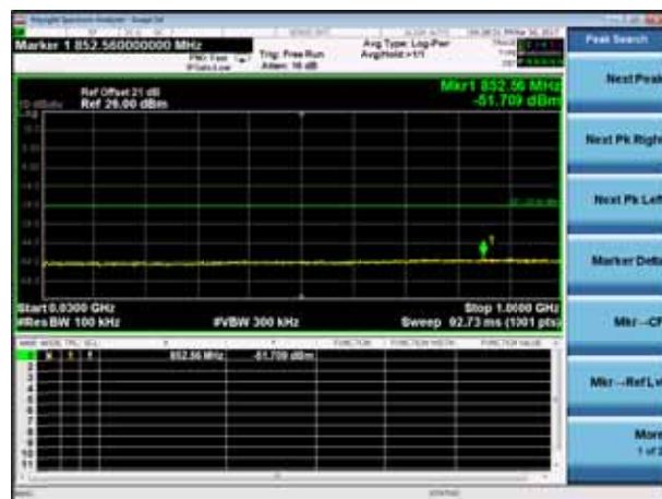
LTE Band 13 BW5M Channel 23230 1RB0
