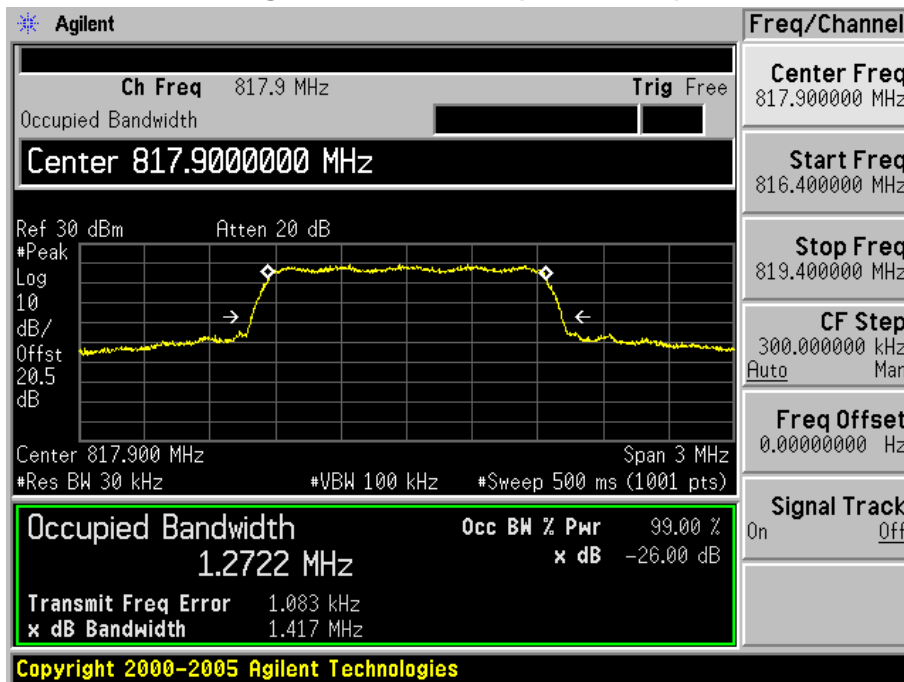
Figure Channel 476 (817.90MHz)
