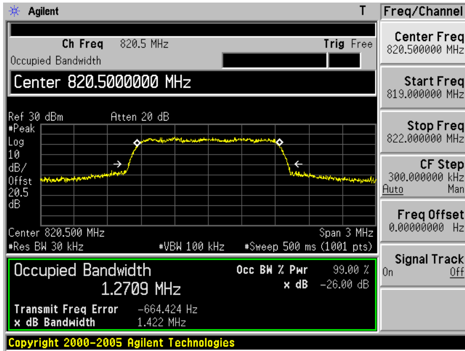
Figure Channel 580 (820.50MHz)
