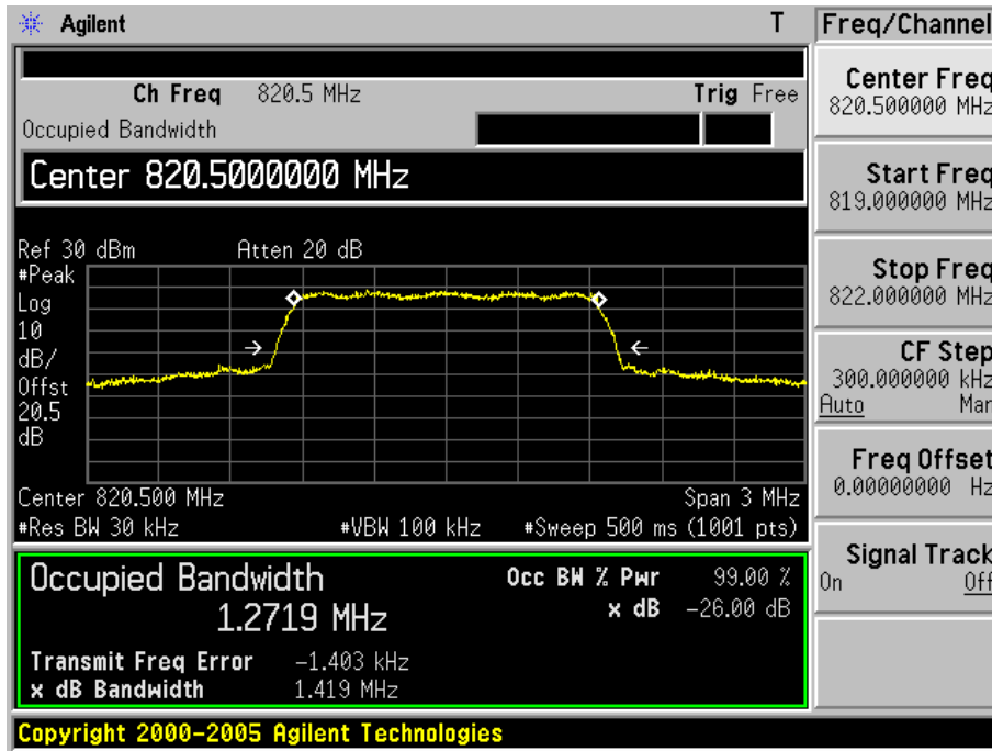
Figure Channel 580 (820.50MHz)
