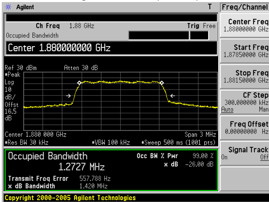
Figure Channel 600 (1880MHz)
