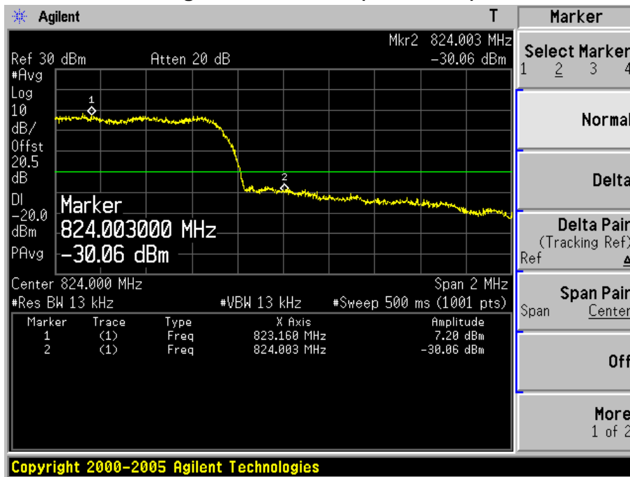
Figure Channel 684 (823.10MHz)
