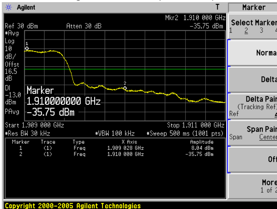
Figure Channel 1175 (1908.75MHz)
