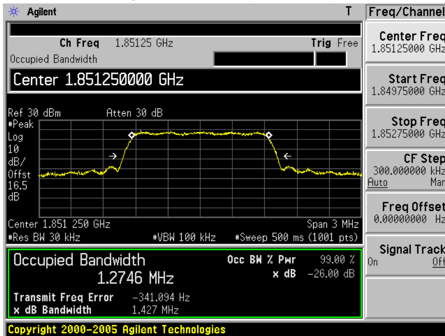
Figure Channel 25 (1851.25MHz)
