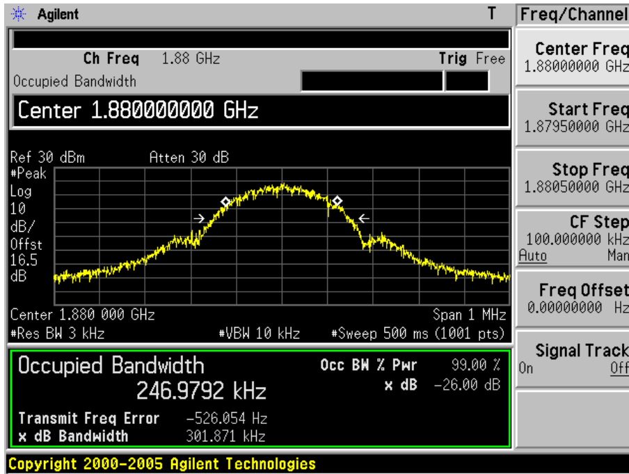
Figure Channel 661 (1880.00MHz)
