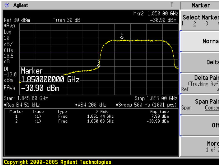
Figure Channel 9262 (1852.40MHz)
