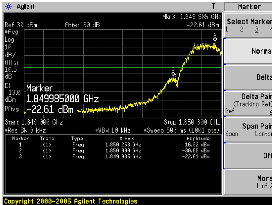
Figure Channel 512 (1850.20MHz)
