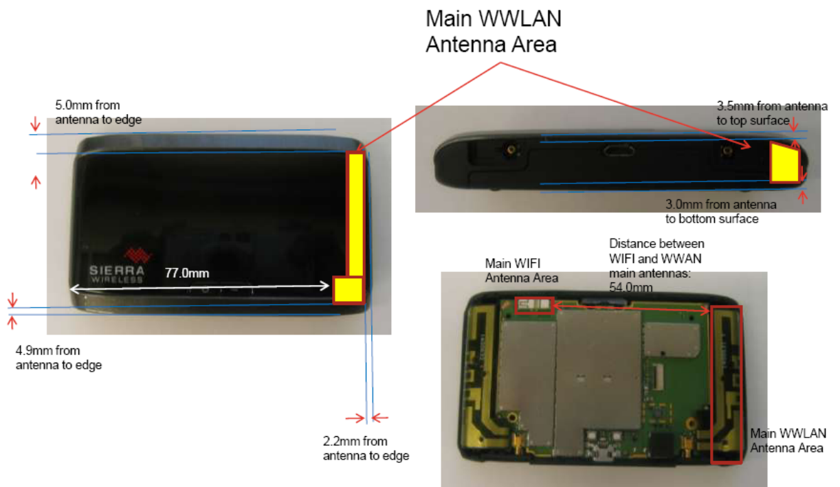
Picture 3: AC763S antenna placement
