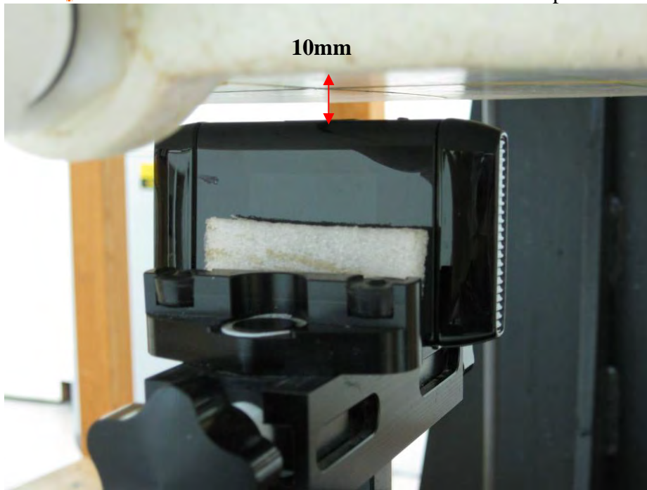
Fig.5 Top side.
