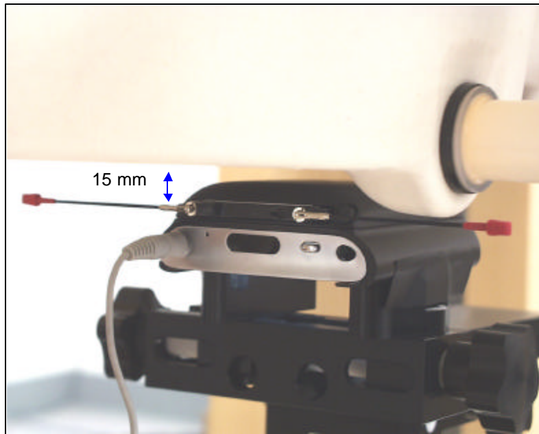
EUT Set-up configuration 2
