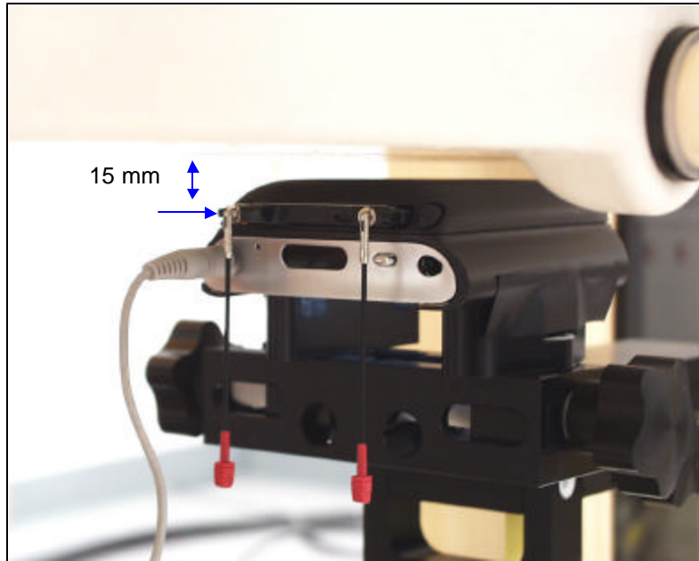
EUT Set-up configuration 1
