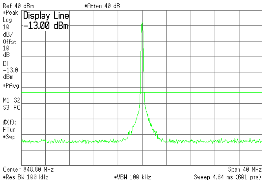
Plot 6.4.8) Out of Band Emissions at Antenna Terminals GMSK, High Channel, 848.8 MHz, TX signal +/- 20 MHz
