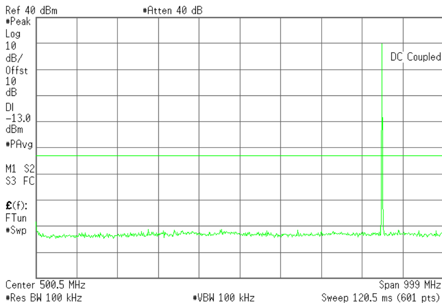
Plot 6.4.17) Out of Band Emissions at Antenna Terminals 8-PSK, High Channel, 848.8 MHz, TX signal +/- 20 MHz
