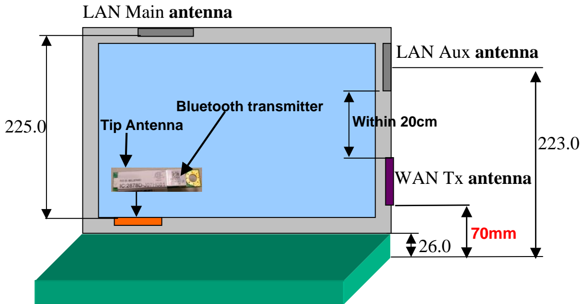
Figure-1 Antenna assembly of Z61m series
