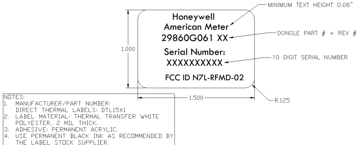
Figure 1 - FCC Label
