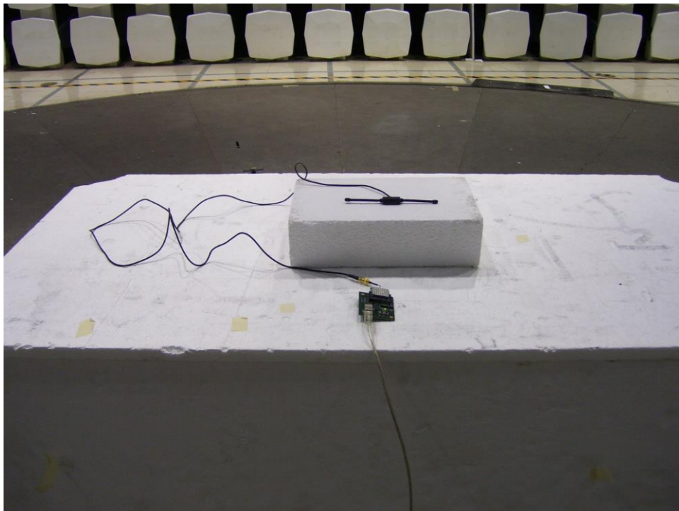
Figure 3: Test Setup View – Setup with Dipole antenna
