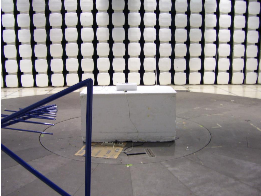
Figure 2: Test Setup View – with Dipole Antenna
