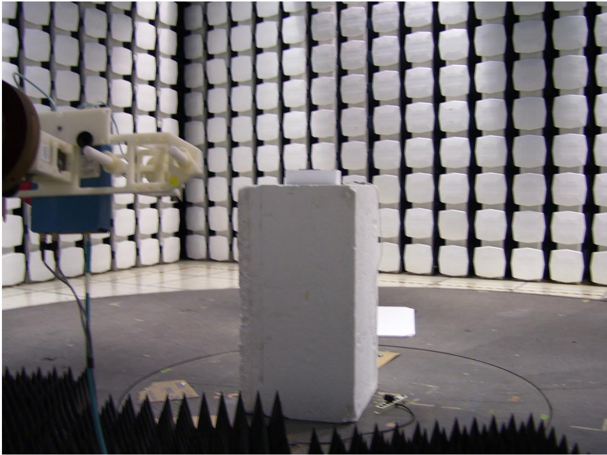
Figure 6: Test Setup View – Over 1 GHz
