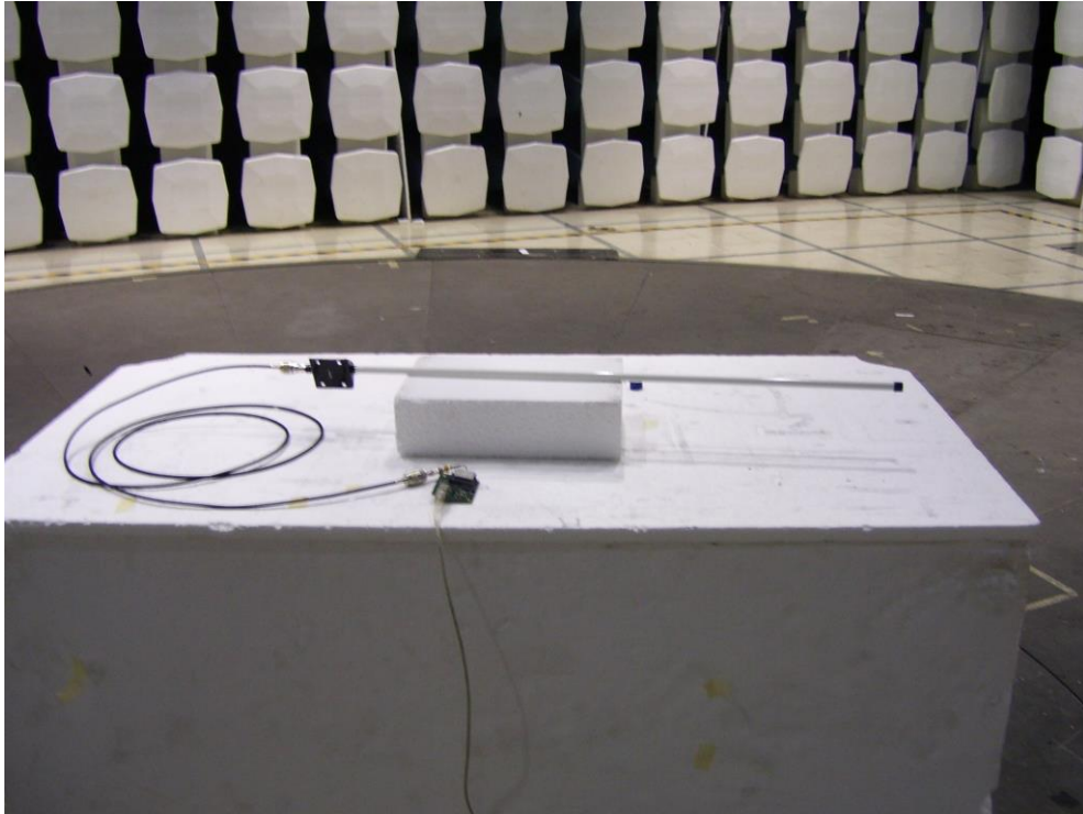
Figure 4: Test Setup View with Monopole antenna
