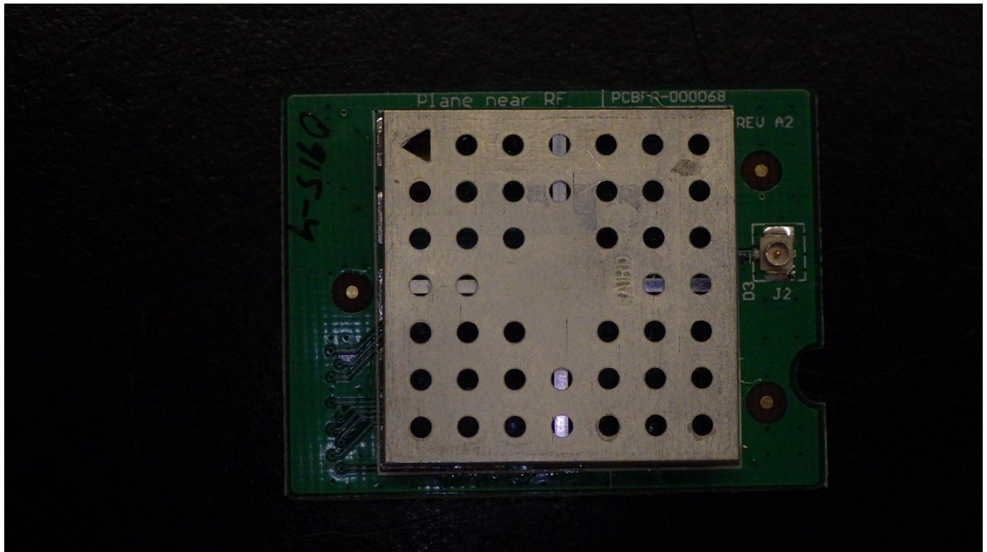
Figure 4: Internal View – Top with RF Shield
