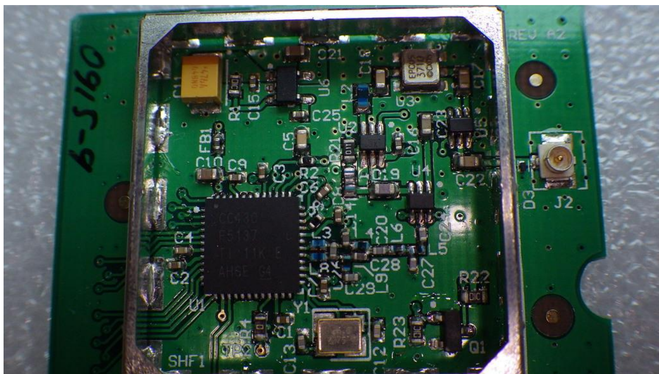
Figure 3: Internal View – RF Shield removed
