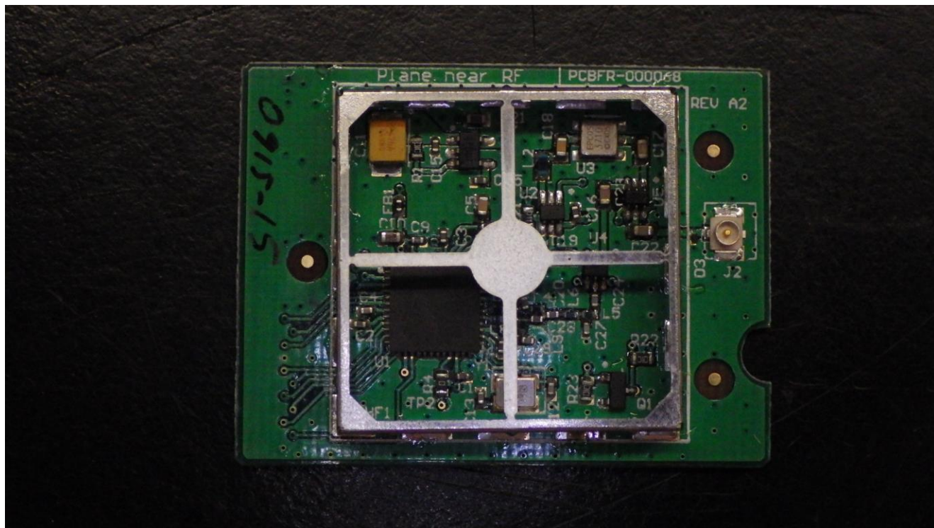
Figure 1: Internal View w/ Remote External Antenna Connection
