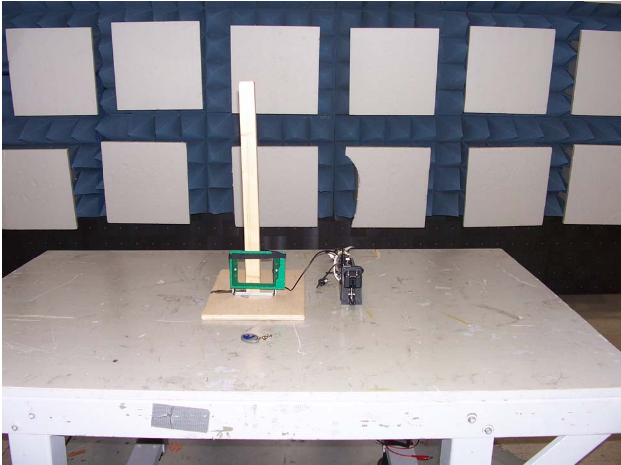
Figure 3 – Typical Radiated Setup Photo of EUT
