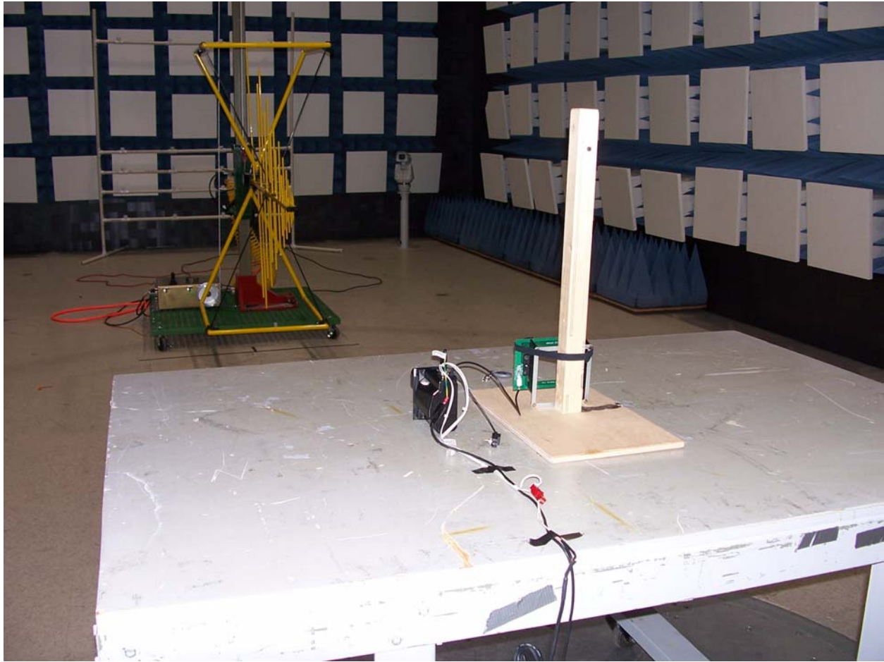
Figure 4 – Typical Radiated Setup Photo of EUT
