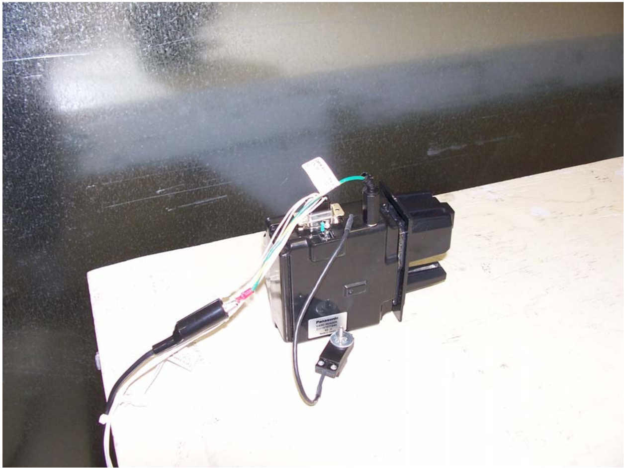
Figure 2 – Conducted Setup Photo of EUT
