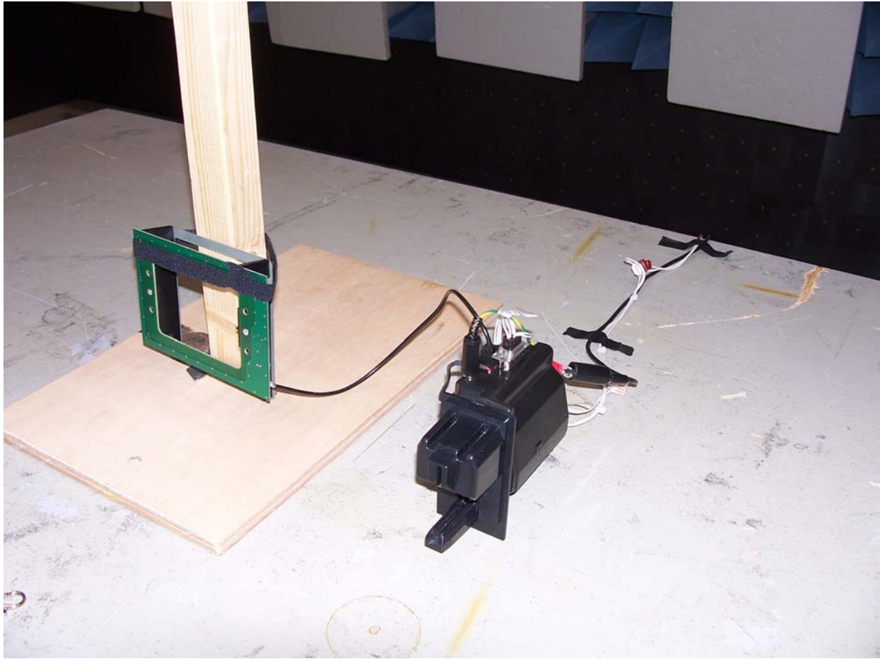
Figure 5 – Typical Radiated Setup Photo of EUT
