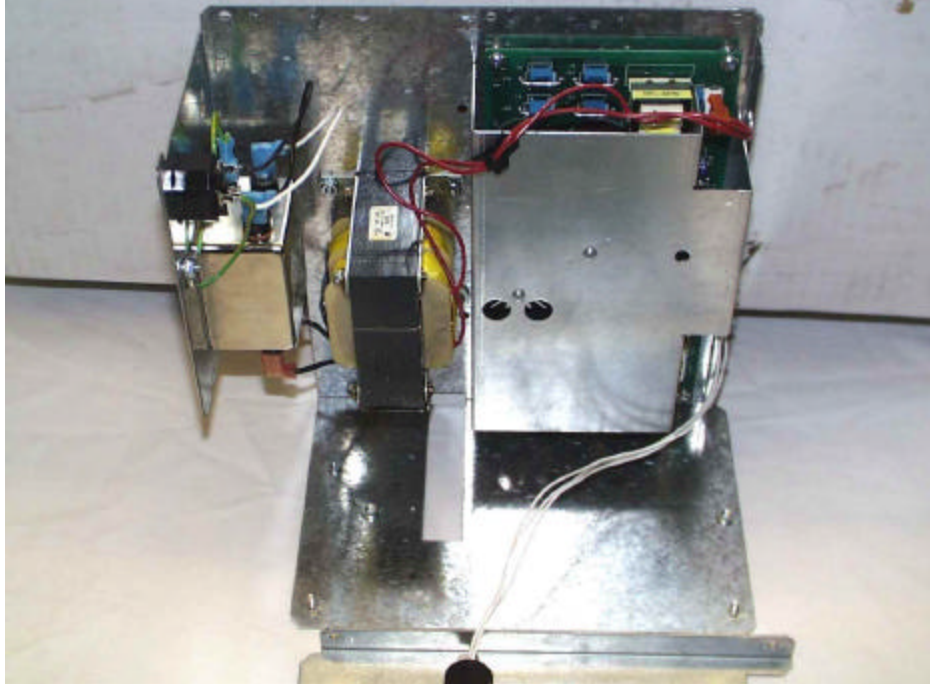
T20606, card cage assembly, power supply view
