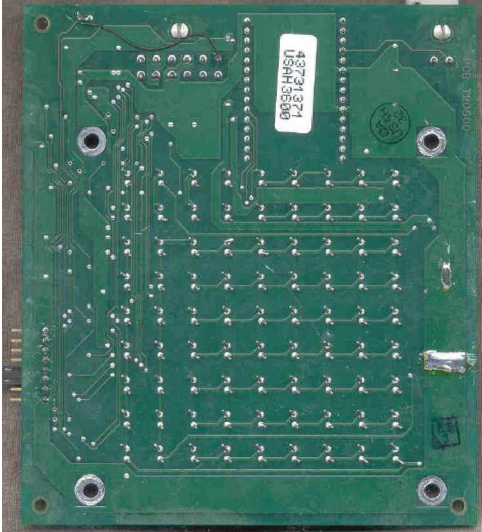
T20601, rear view
