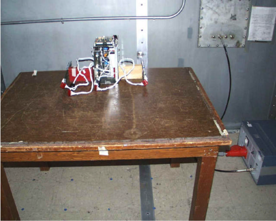
Conducted Emissions Test Setup – Encore Configuration
