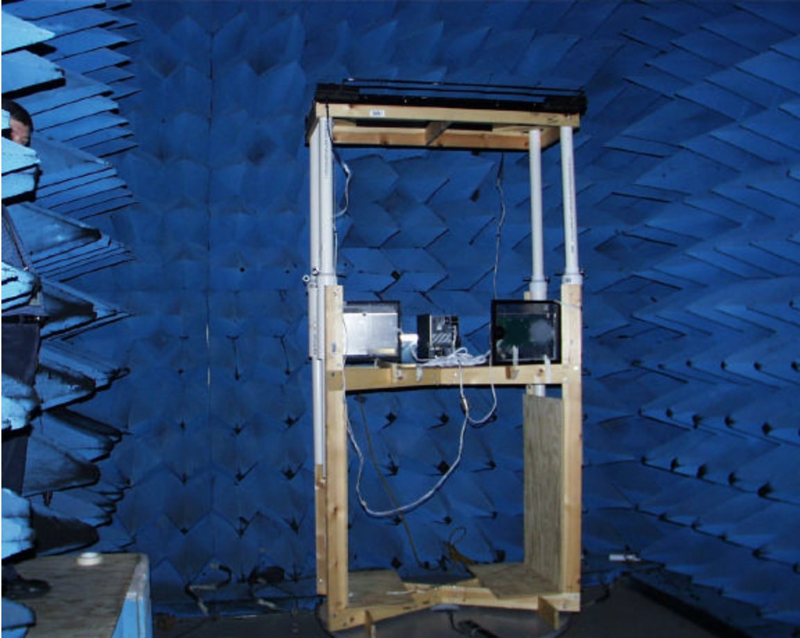
Radiated Emissions Pre-scan (Anechoic) Test Setup – Advantage Configuration
