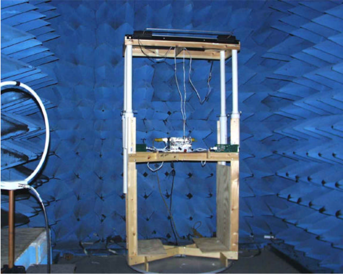
Radiated Emissions Pre-scan (Anechoic) Test Setup – Encore Configuration
