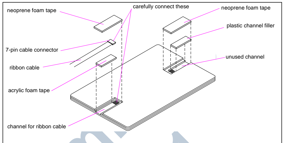
Figure: Connecting to Mat Reader - Low Frequency
