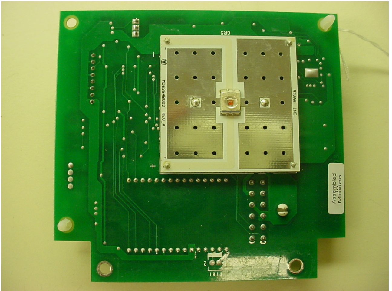
Figure 3: PCB - Back
