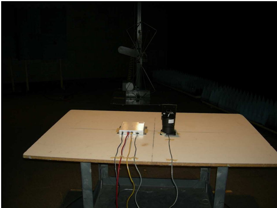
Figure 2: Radiated Emissions Test Setup – 45 Degree Angle
