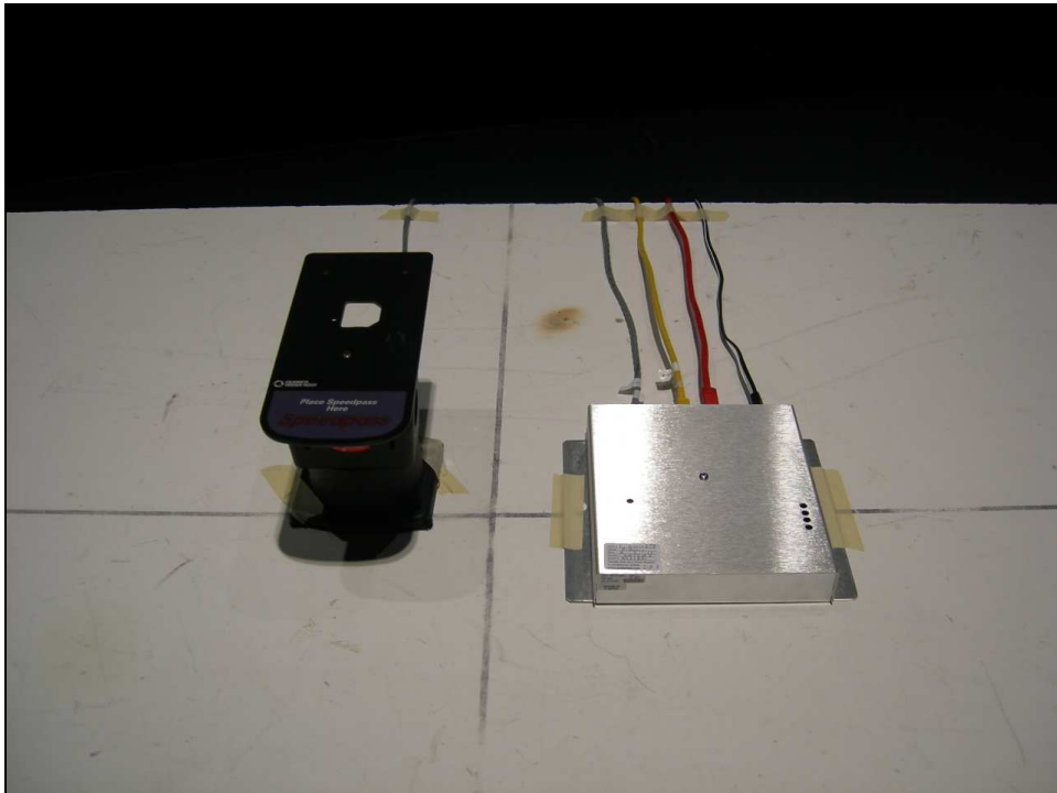
Figure 3: Radiated Emissions Test Setup – Flat Orientation
