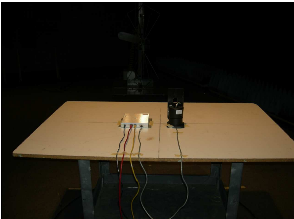
Figure 6: Radiated Emissions Test Setup – Upright Orientation
