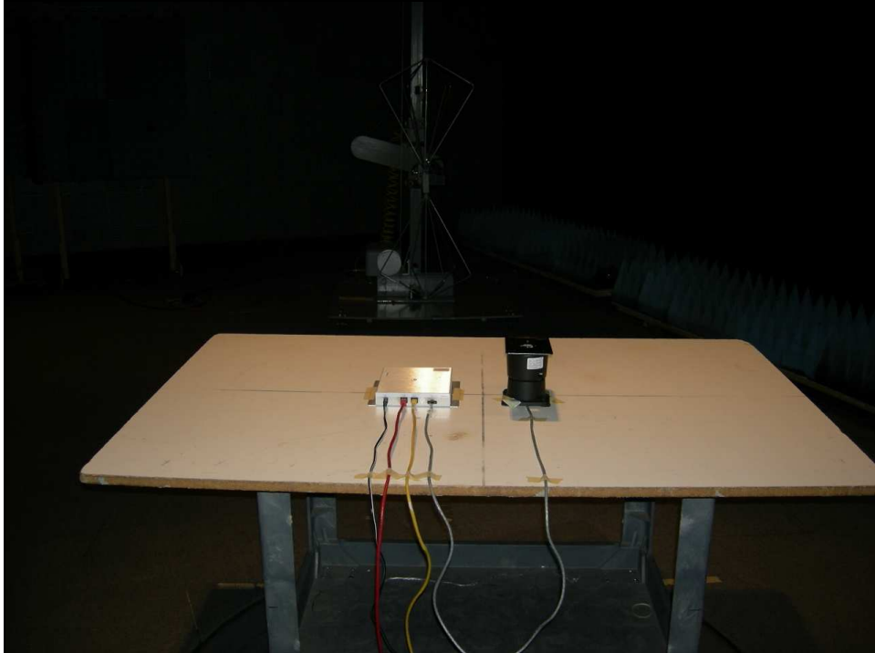
Figure 4: Radiated Emissions Test Setup – Flat Orientation
