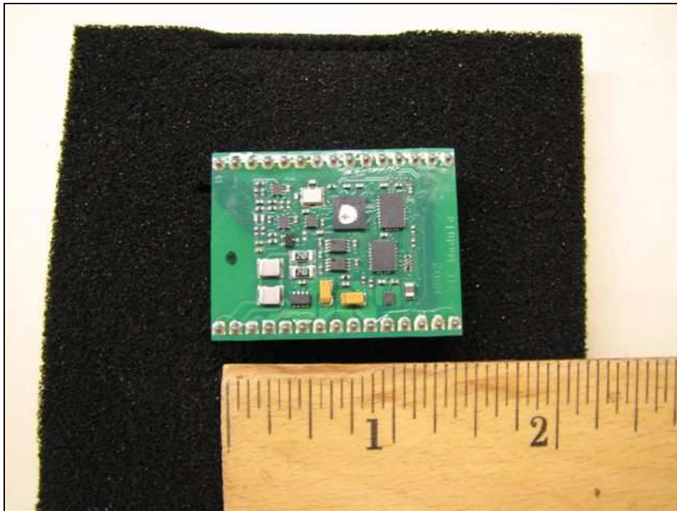
Figure 3: Internal Photo – Transceiver Module
