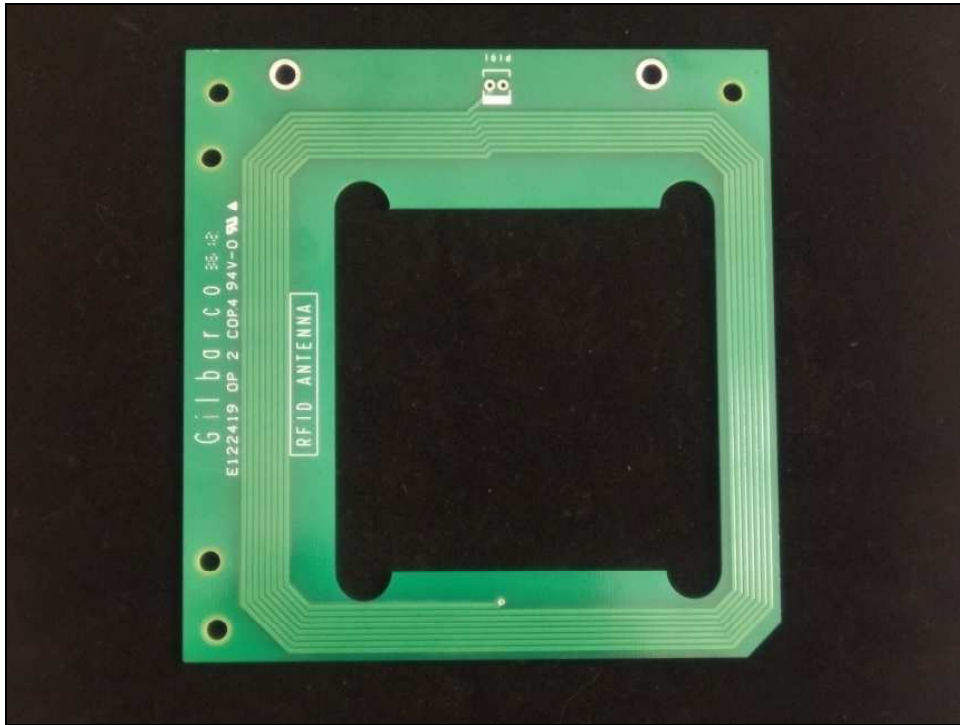
Figure 5: Internal Photo – Antenna
