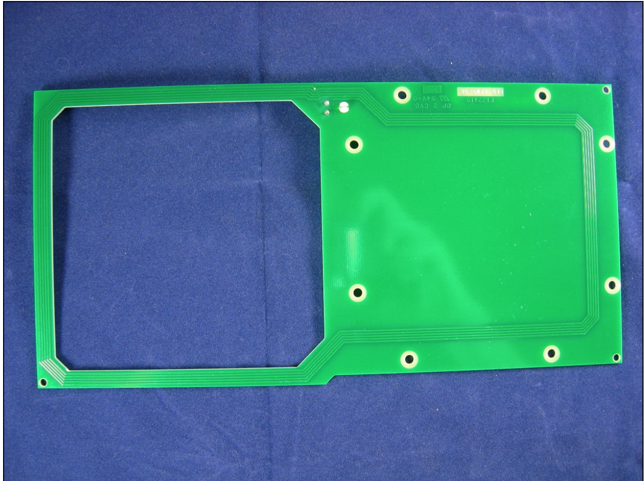
Figure 7: Internal Photo – Antenna PCB
