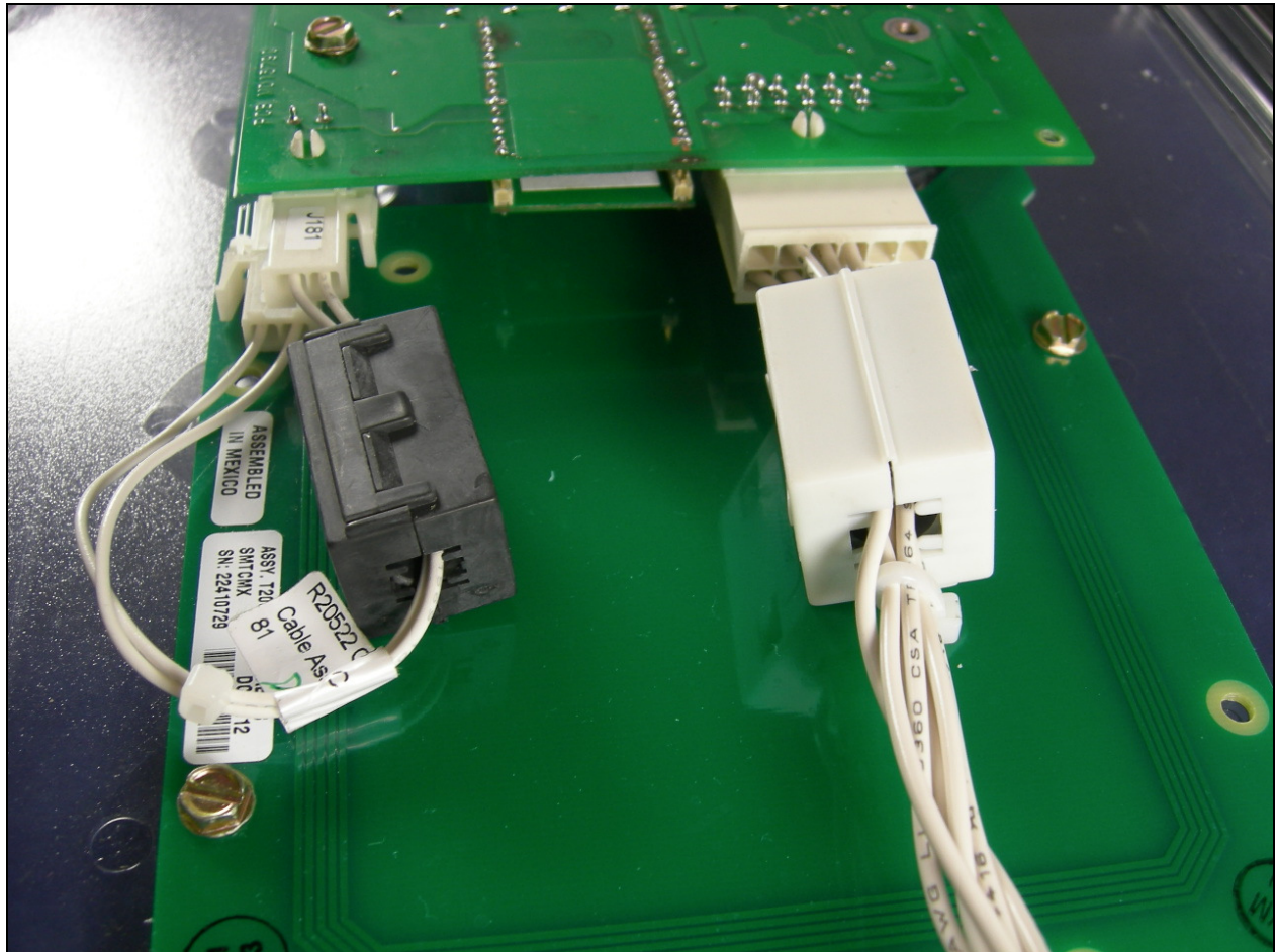
Figure 2: Internal Photo (Modifications)
