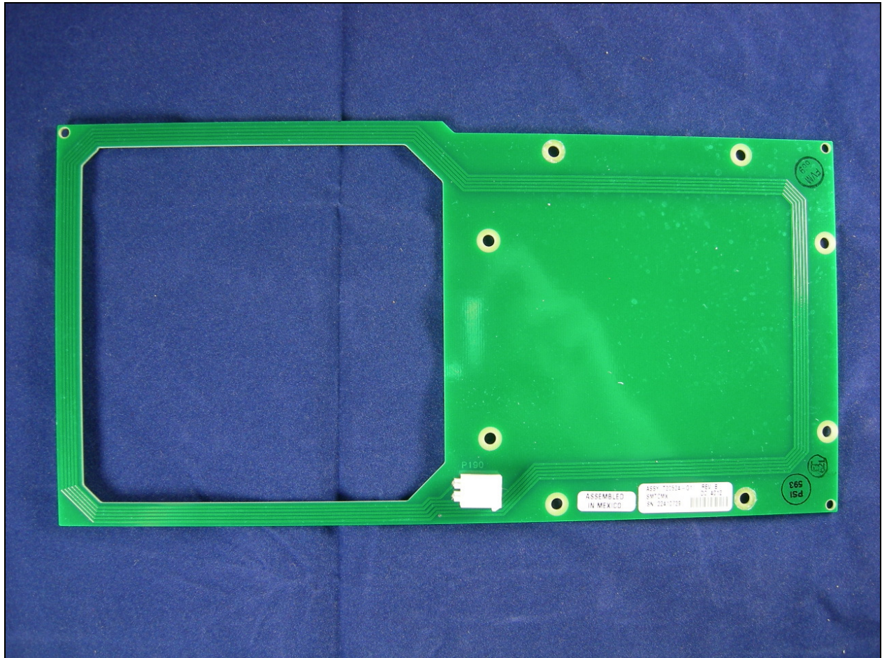
Figure 6: Internal Photo – Antenna PCB
