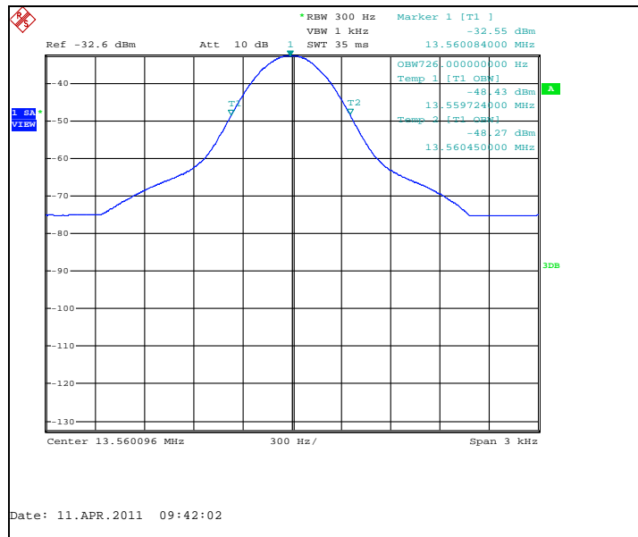
Figure 7.4.2-2: Occupied Bandwidth – 99%
