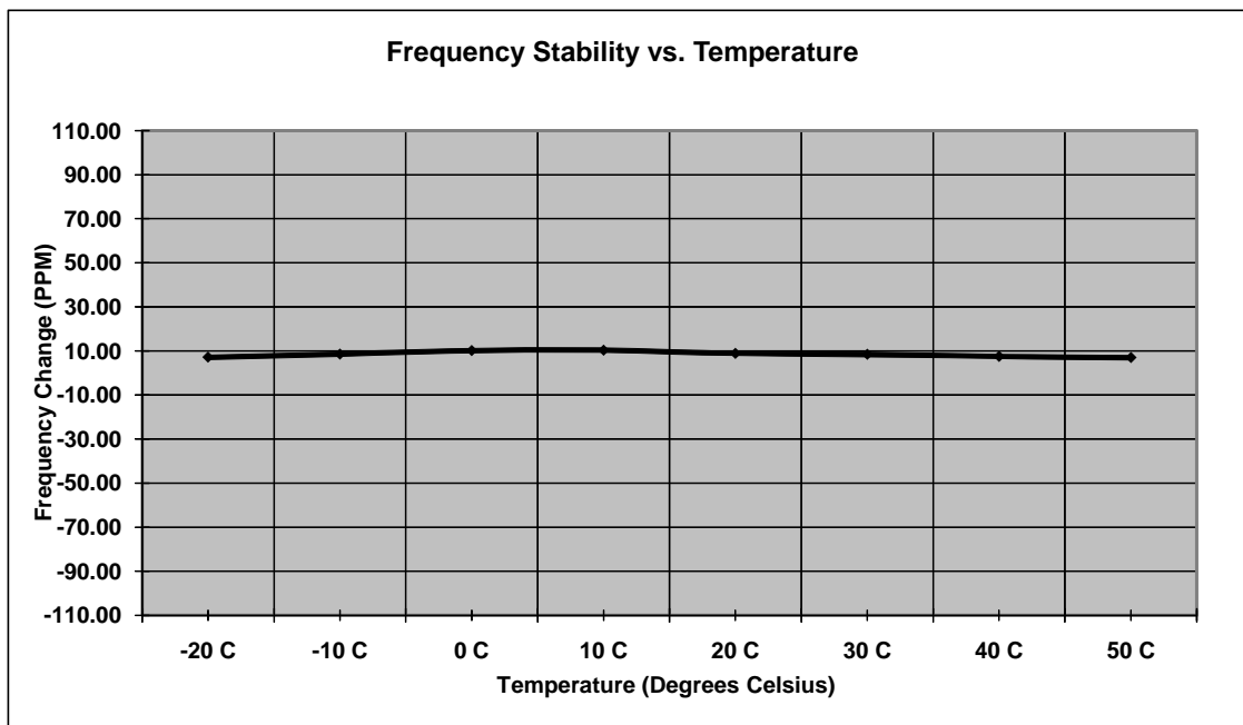
Figure 7.5.2-1: Frequency Stability
