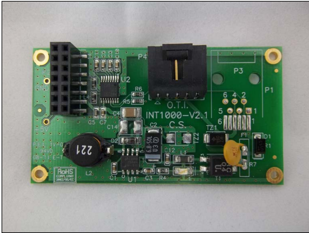
Figure 7: Internal Photo
