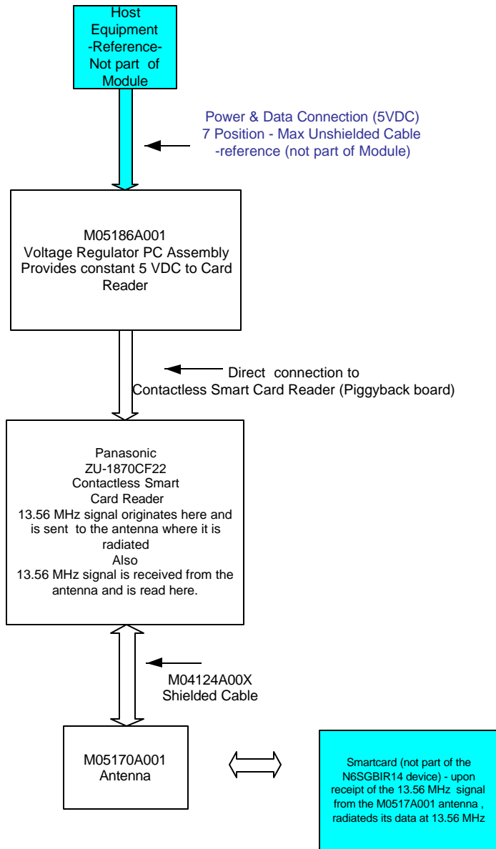
Figure 1: Block Diagram of the Contactless Smart Card Reader System
