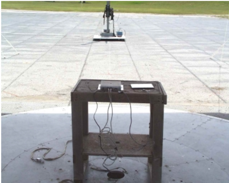
Radiated Emissions OATS Test Setup (30 MHz to 1 GHz)
